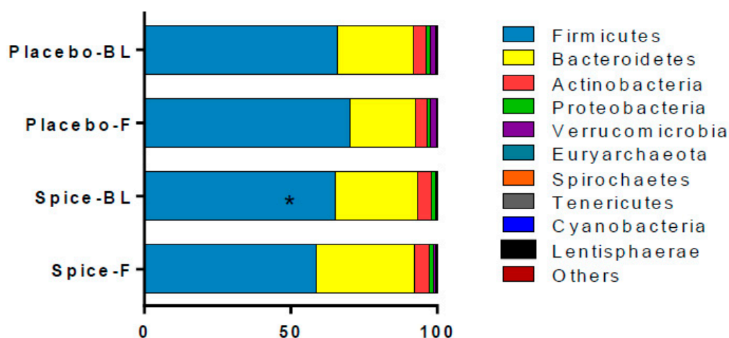
Figure 4. Comparison of fecal microbiota in subjects supplemented with placebo and mixed spices capsules. Bar graph shows the relative abundance of phylum in subjects supplemented with placebo ( n = 15 ) or mixed spices ( n = 14 ) at baseline and after 2 week intervention. Each color within the bar graphs represents a phylum, with area of the color proportional to relative abundance. PBL, placebo group at baseline; PF, placebo group at follow up; SBL, spice group at baseline; SF, spice group at follow up. Data are means \pm standard errors (SE). Significant difference in abundance between placebo and spice group is indicated by * p < 0.05 .
