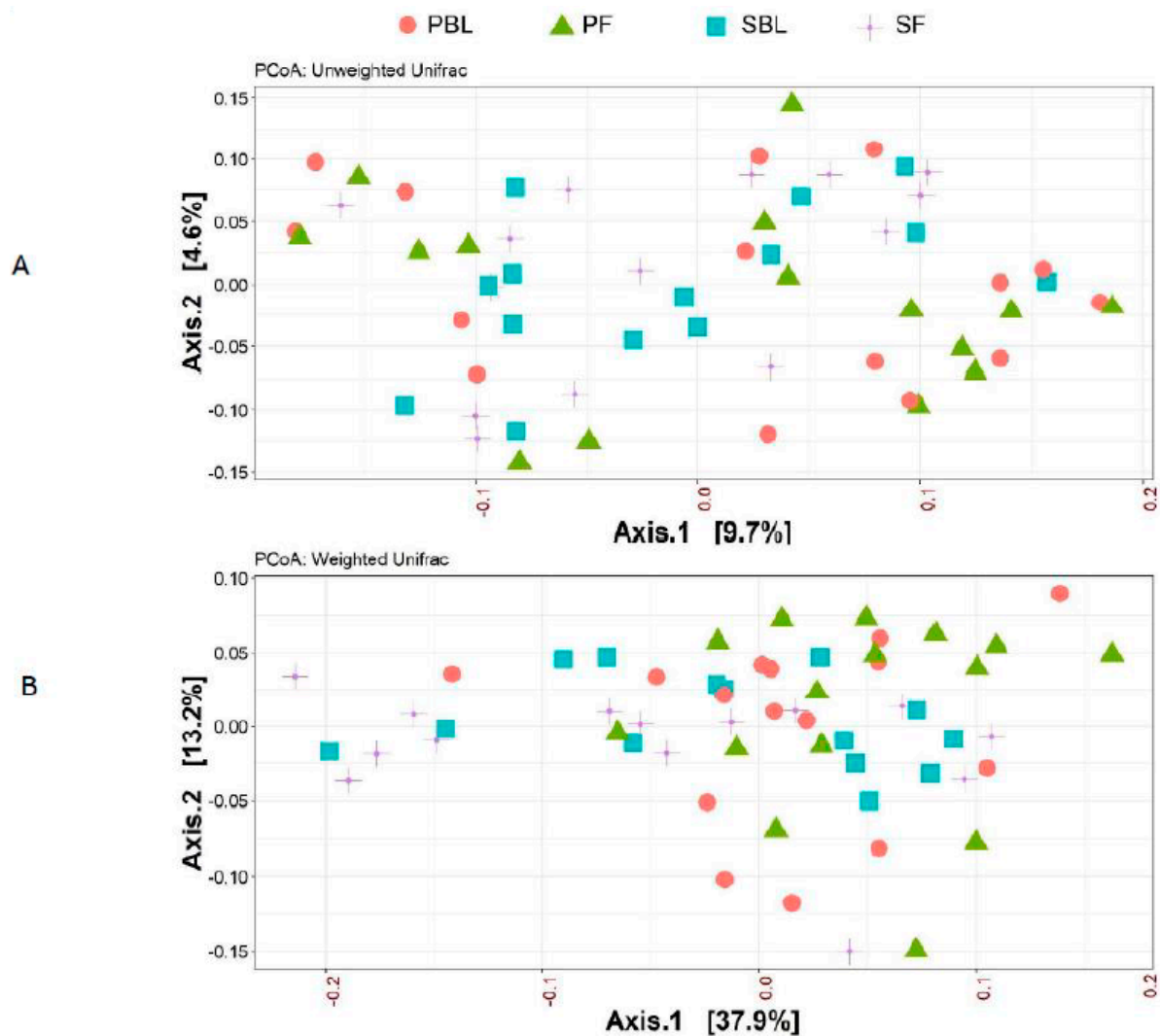
Figure 3. Beta-diversity between placebo group and spice group. Principal coordinate analysis (PCoA) plots of all fecal samples from 29 subjects in two groups at baseline and 2 week follow up. Red circle and green triangle represent participants in PBL and PF, blue square and purple cross represent participants in mixed SBL and SF, respectively. (A) Unweighted UniFrac. (B) Weighted UniFrac. Axis 1, principal coordinate 1; axis 2, principal coordinate 2. PBL, placebo group at baseline; PF, placebo group at follow up; SBL, spice group at baseline; and SF, spice group at follow up.
