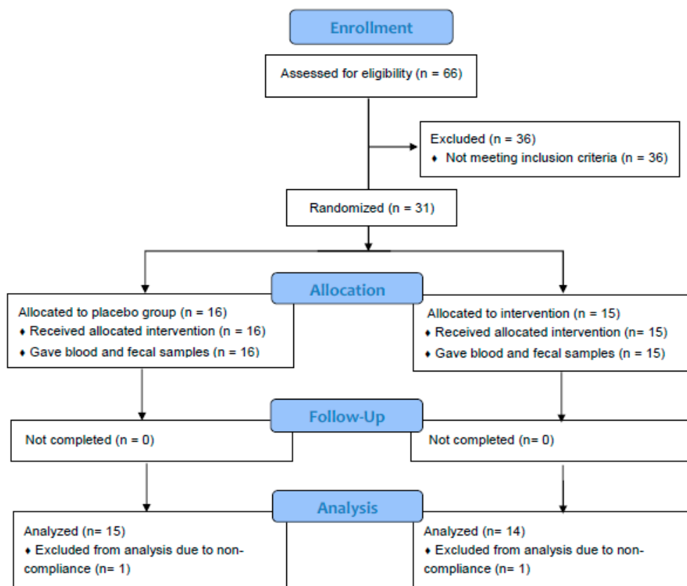
Figure 1. Flowchart of study subjects. A total of 31 subjects were randomized and completed study. Twenty-nine subjects were included in data analysis. Two subjects were excluded due to non-adherence to protocol.
