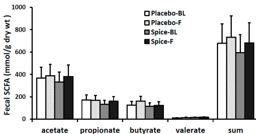
Figure 5. Fecal short-chain fatty acid production in subjects supplemented with placebo ( n = 15 ) or mixed spices ( n = 14 ) at baseline and after 2 week intervention. Data are means \pm standard errors (SE). BL, baseline; F, follow up.
