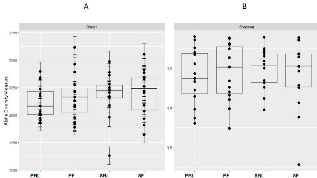
Figure 2. Within-sample alpha-diversity of fecal of 29 subjects collected at the baseline and 2 weeks. Calculation of the alpha-diversity for each sample for evaluating species richness and diversity by using Chao1 (A) and Shannon (B) effective indices. The diversity of a microbial profile for a certain index is the number of different species related to abundance and richness. PBL, placebo group at baseline; PF, placebo group at follow up; SBL, spice group at baseline; and SF, spice group at follow up.
