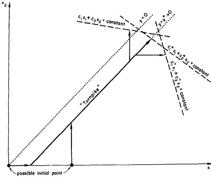
FIG. 4. Turnpike in x_1x_2 plane. Optimal trajectories shown for two possible initial points and three possible ratios of objective function weighting coefficients.
