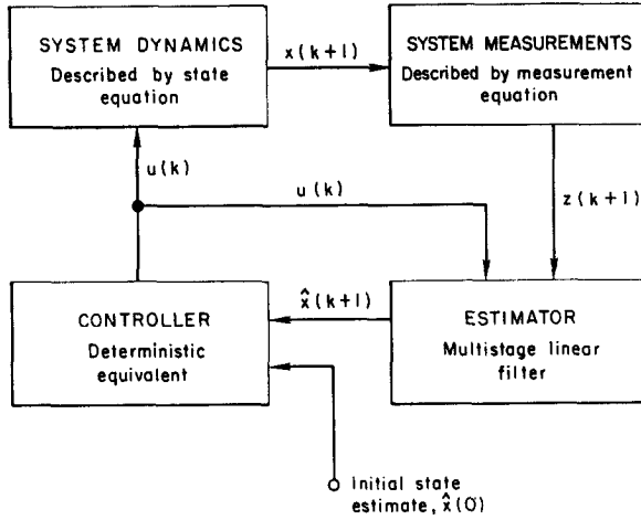
FIG. 7. Block diagram of system with estimator and controller.
