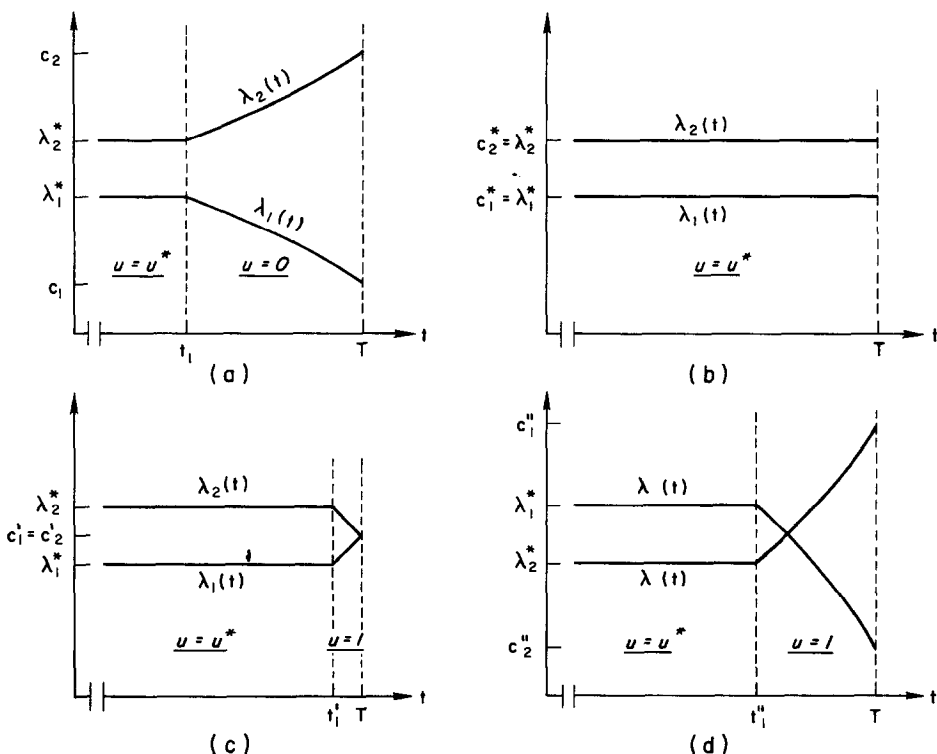
FIG. 5. Adjoint variables near end of study period for four different c_1/c_2 ratios.
