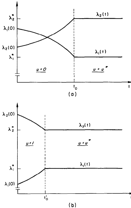
FIG. 6. Adjoint variables near beginning of study period for two different initial points. Case (a) y_0 > y^* and Case (b) y_0 < y^* .
