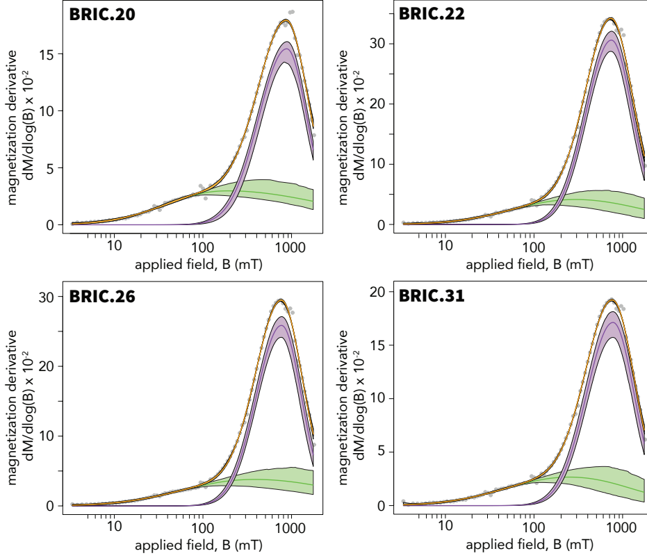
Figure 4. Coercivity spectra developed from backfield demagnetization curves on BRIC intraclast specimens with the points being the data. The data were modeled using log-Gaussian distributions implemented with the Max UnMix software package (Maxbauer et al., 2016). The coercivity spectra can be well-explained with two distributions: the higher coercivity distribution in purple and the lower coercivity distribution in green. The shaded areas represent 95% confidence intervals for the modeled components.
