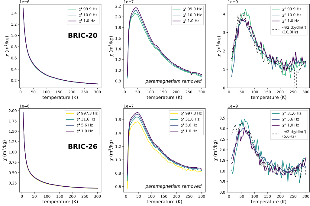
Figure 5. Frequency and temperature dependence of magnetic susceptibility ( \chi ) for BRIC-20 and BRIC-26 from 10 to 300 K. The left panels show the in-phase susceptibility which is dominated by the paramagnetic component of the samples. In the middle panels, this paramagnetic component has been removed by creating a Curie-Weiss law model and subtracting it from the in-phase susceptibility data. Strong frequency dependence over the whole temperature range suggests a broad size distribution of nanoparticles (e.g. (Jackson & Swanson-Hysell, 2012)). The right panels show the out-of-phase (quadrature) susceptibility as well as the \pi/2 relationship of \chi''[\text{viscosity}] = -(\pi/2)(\partial\chi'/\partial\ln f) where f =frequency. These data document the presence of viscous superparamagnetic particles.
