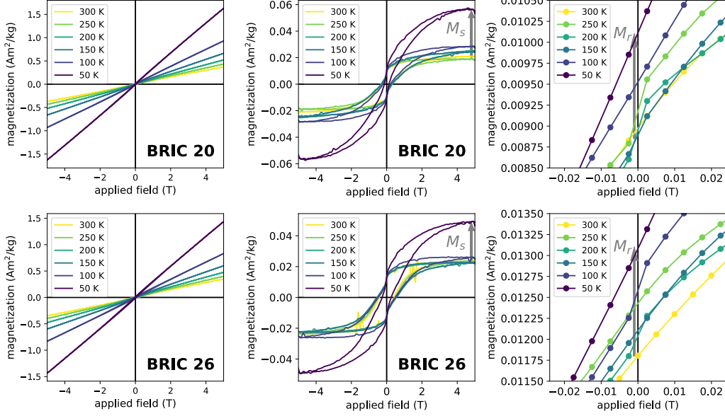
Figure 6. Hysteresis loops measured from room temperature (300 K) down to 50 K for siltstone intraclast samples. The left panels are the raw uncorrected loops, the center panels remove the paramagnetic contribution using the methods of Jackson and Solheid (2010) and the right panels zoom-in on applied fields close to 0 to illustrate the progressive increase in remanent magnetization ( M_r ) as temperature decreases.
