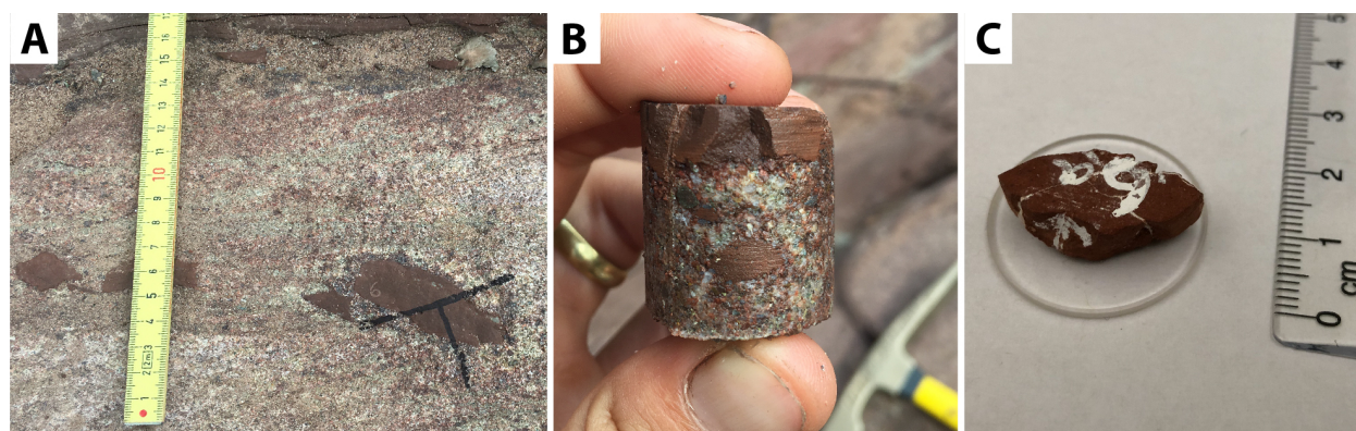
Figure S2. Photos of intraclast BRIC-6: in the field within coarse sandstone (A), at the top of an oriented drill core sample (B) and prepped with the matrix sandstone removed on a quartz glass disk (C). The numbered divisions on the rulers in A and C are both in centimeters. Panel A shows multiple siltstone intraclasts. The one marked with the \lambda is the clast sampled as BRIC-6.
