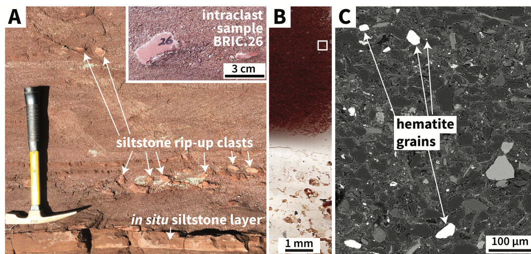
Figure 1. A: Siltstone intraclasts within the Freda Formation. The field photo shows an intact layer of siltstone below the hammer head which is topped by a bed of trough cross-stratified coarse-grained sandstone with horizons of siltstone intraclasts. The hammer is 40 cm long. The inset photo is of an individual intraclast that was sampled as BRIC.26. B: A scan of a 30 \mu\text{m} -thick thin section of the BRIC.26 intraclast (upper half of image) and the coarse sand matrix (lower half of image). The red color of the intraclast is due to pigmentary hematite. C: Backscatter electron image of the siltstone clast from the region of the white box in B. The light-colored detrital grains that are labeled with arrows (light due to iron's high atomic number) were confirmed to be hematite through electron backscatter diffraction.
