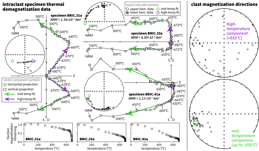
Figure 2. Paleomagnetic data from intraclasts reveal a mid-temperature component that typically unblocks prior to 655°C and a high-temperature component that typically unblocks between 655°C and 687°C. These components are present as varying fractions of the overall remanence as seen in the three individual clasts shown here on vector component plots and measurement-level equal area plots in tilt-corrected coordinates (developed using PmagPy; (Tauxe et al., 2016)). The direction of the mid-temperature component is shown as green arrows on the vector component plots and green circles on the equal area plots while the high-temperature component is shown with purple symbols. The mid-temperature component has a similar direction among the clasts as can be seen on the component directions equal area plots (tilt-corrected mean declination: 251.8, inclination: -12.4, \alpha_{95} : 6.6). In contrast, the high-temperature component directions are dispersed.
