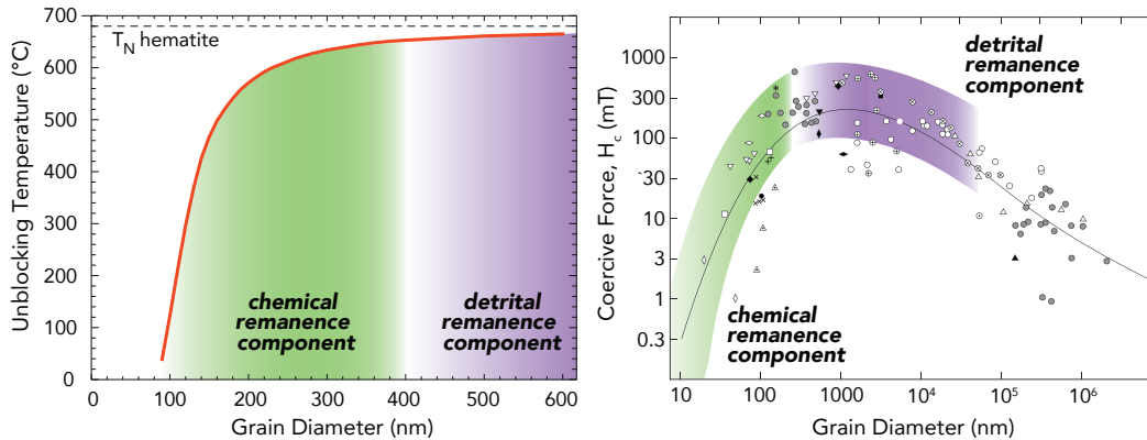
Figure 8. Left: Calculated unblocking temperatures using Néel thermal relaxation theory of idealized spherical hematite grains using a thermal fluctuation rate of 10^{10} \text{ s}^{-1} and a relaxation time of 5 minutes for comparison to thermal demagnetization data (modified from (Swanson-Hysell et al., 2011)). The unblocking temperatures of the mid-temperature chemical component (green) and the high-temperature detrital component (purple) are shown and can be used to infer grain size. The Néel transition temperature ( T_N ) is shown with a dashed line. Right: Compilation of coercivity data from hematite as a function of grain diameter from (Özdemir & Dunlop, 2014). The higher coercivity population from Fig. 4 corresponds to the larger grain sizes than the lower coercivity component associated with the chemical remanence.
