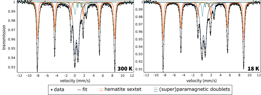
Figure 7. Mössbauer spectra developed at room temperature (300 K) and low temperature (18 K) on a powder of intraclast sample BRIC.22. Data are shown as dots with the black line representing a model fit. The sextet portion of the fit is shown with the red and yellow curves (representing the spread in hyperfine splitting resulting from a natural population) and is diagnostic of hematite. The central peak is comprised of doublets dominated by \text{Fe}^{3+} . The height of the hematite sextet relative to the central peak is slightly higher in the low temperature experiment likely due to ordering of the smallest hematite nanoparticles.
