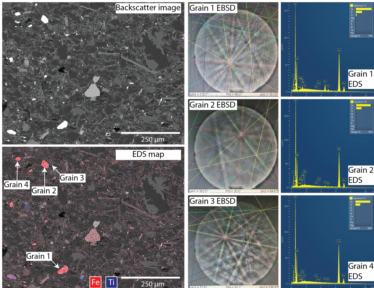
Figure S3. Scanning electron microscopy images and data for sample BRIC-26. The energy-dispersive X-ray spectroscopy (EDS) map shows the distribution of Fe and Ti for the same view as the backscatter image. This map reveals both micron-scale oxide grains (hematite, ilmenite and \text{TiO}_2 ) and disseminated iron within clays and the matrix. EDS spectrum are shown for individual labeled grains as are electron backscatter diffraction (EBSD) images matched with the hematite pattern which identifies the grains. These techniques, along with optical reflected light microscopy, were used to identify the grains labeled as hematite in Figure 1 of the main text.
