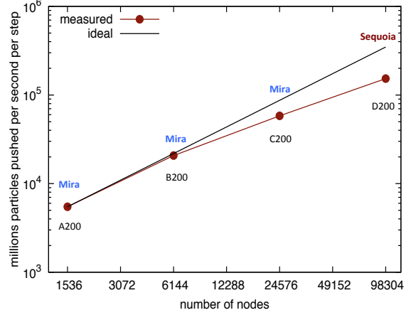
Figure 5: GTC-P (new) weak scaling with respect to “the number of particles pushed per second per step” with different size devices on BG/Q. Particle numbers in one process is about 404,487. n_{toroidal}=64 , n_{pe\_radiald}=2 , n_{radiald}=8, 32, 128 , and 512 for A,B,C and D respectively. The D size was performed on Sequoia, while the others were on Mira. Experiments use 1 process/node and 64 threads/process.
