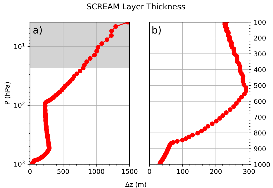
Figure 1. SCREAM grid spacing. Panel (a) shows the complete vertical grid using logarithmic pressure to emphasize the upper atmosphere. Panel (b) zooms in on the troposphere using linear pressure spacing to emphasize lower levels. The sponge layer is indicated by gray-shading.
