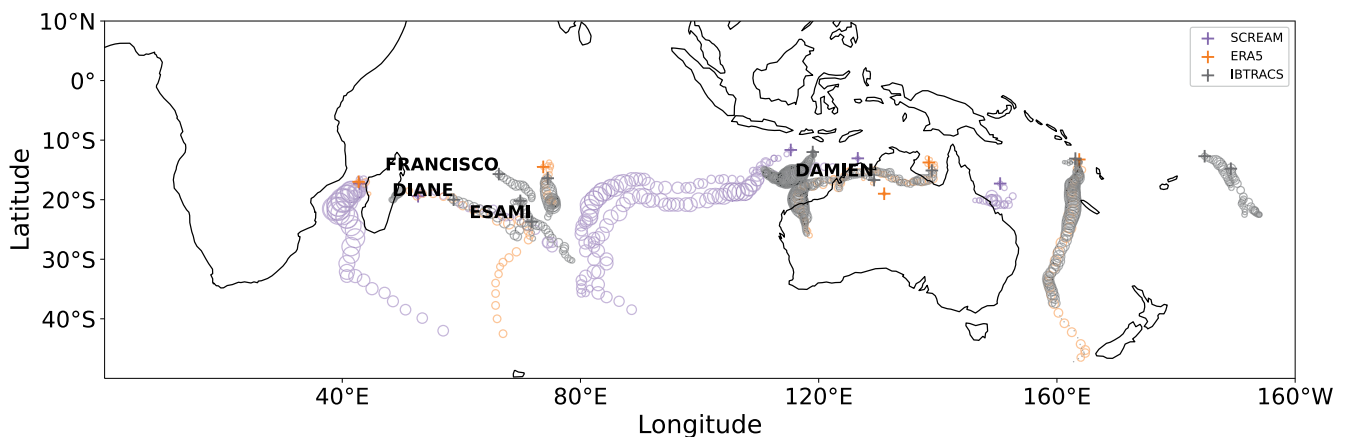
Figure 18. Tracks of tropical storms from IBTrACS (gray) and identified by the Tempest Extremes algorithm in SCREAM (purple) and in ERA5 (orange) between January 20 and February 28, 2020. Starting location is indicated with a plus (+).
