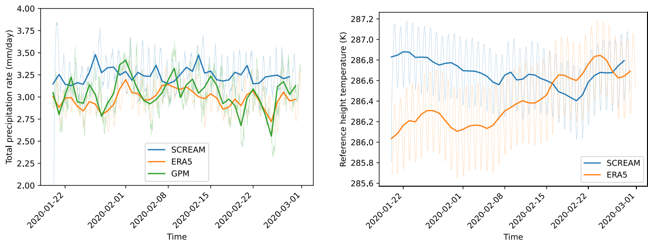
Figure 5. Fifteen minute (thin curves) and daily mean (thick curves) time series of global-average precipitation (left) and 2 m temperature (right) for the duration of the DYAMOND2 simulation.
