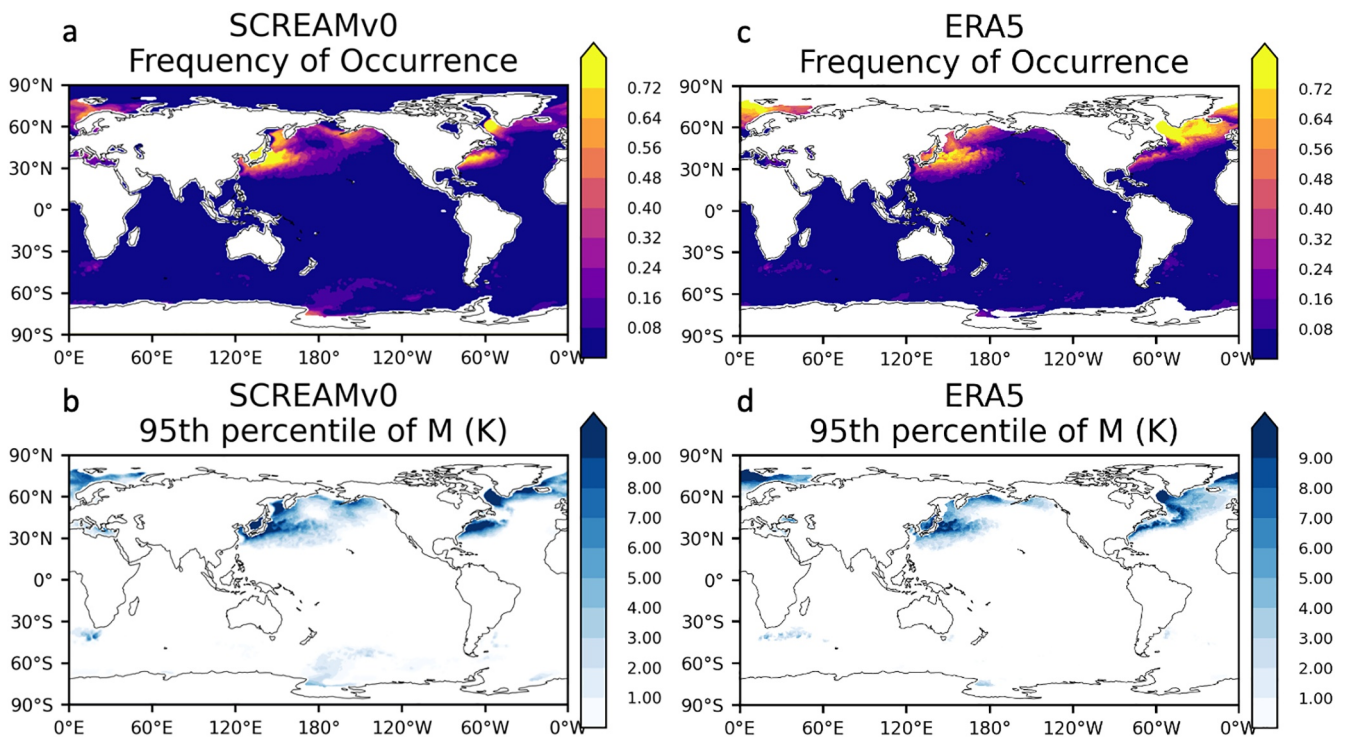
Figure 25. Frequency of cold air outbreaks (based on the M of Fletcher et al. [2016]) in SCREAM over the month of February 2020 in SCREAM (a) and in ERA5 (c). Also shown is the 95th percentile value of M (including non-cold air outbreak instances) over the same period in SCREAM (b) and ERA5 (d).
