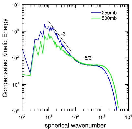
Figure 2. Compensated kinetic energy spectra ( E(k)k^{5/3} ) at 500 and 250 hPa from days 23 to 24 of the simulation. The black lines show idealized E(k) \approx k^{-3} and E(k) \approx k^{-5/3} scalings. See text for details.
