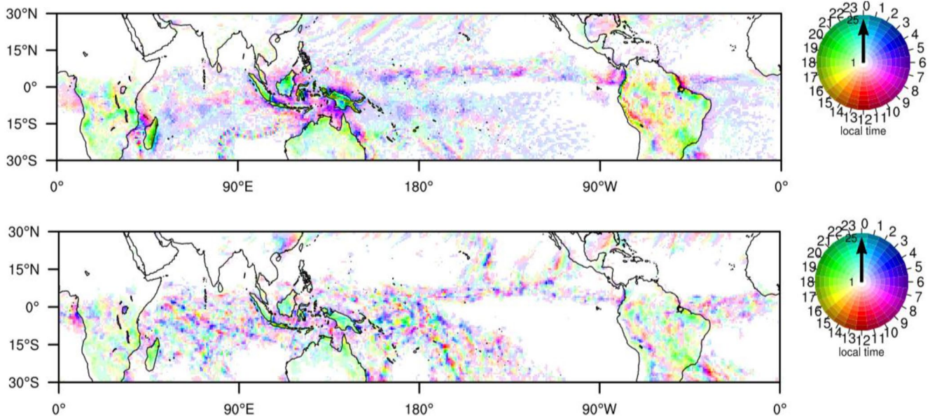
Figure 15. Diurnal cycle of precipitation averaged over the last 30 days of the SCREAM run (top) and GPM observations (bottom). Hue indicates time of peak precipitation and intensity indicates diurnal amplitude. Amplitudes less than 1 \text{ mm day}^{-1} are colored white and colors saturate at 25 \text{ mm day}^{-1} .
