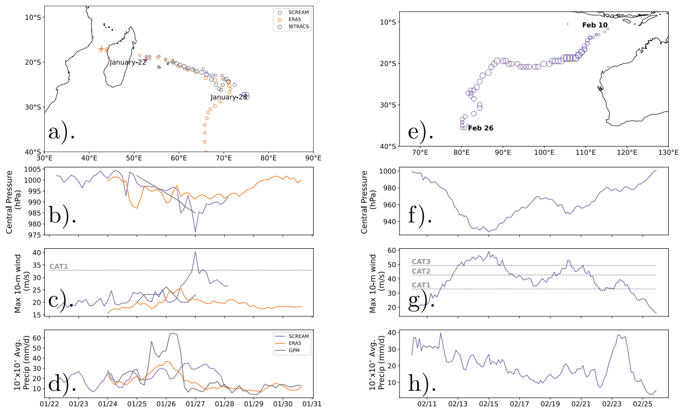
Figure 19. (a) Tracks of the tropical storm Diane from IBTrACS (gray) and as identified by the Tempest Extremes algorithm in SCREAM (purple) and in ERA5 (orange). Starting location is indicated with a + symbol. Shown below the tracks are time evolution of the storm's minimum central pressure (b), maximum 10-m wind speeds within 5° of the storm center (c), and area-averaged precipitation rate (d). (e–h) Same as (a–d) but for February 10 tropical cyclone in SCREAM simulation. No observational equivalent is shown, because it is outside the period of predictability.
