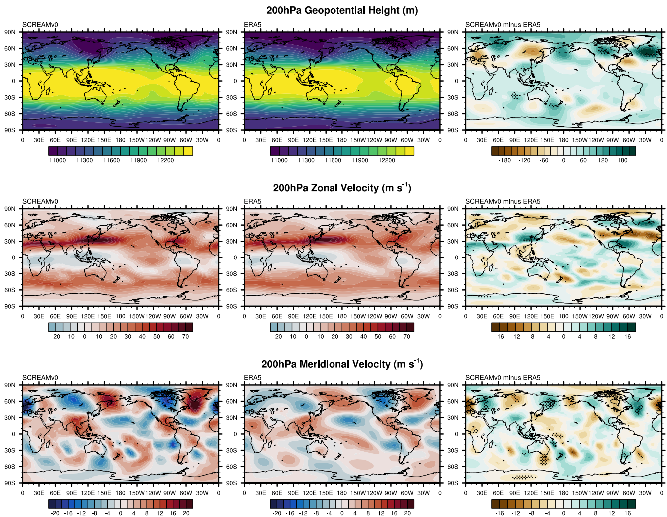
Figure 8. 200 hPa geopotential height (top), zonal wind speeds (middle), and meridional wind speeds (bottom) averaged over the last 30 days of the simulation. Stippling in the difference plots (right panels) indicates regions where SCREAM falls outside the range of mean values for all years in ERA5 1979–2020.
