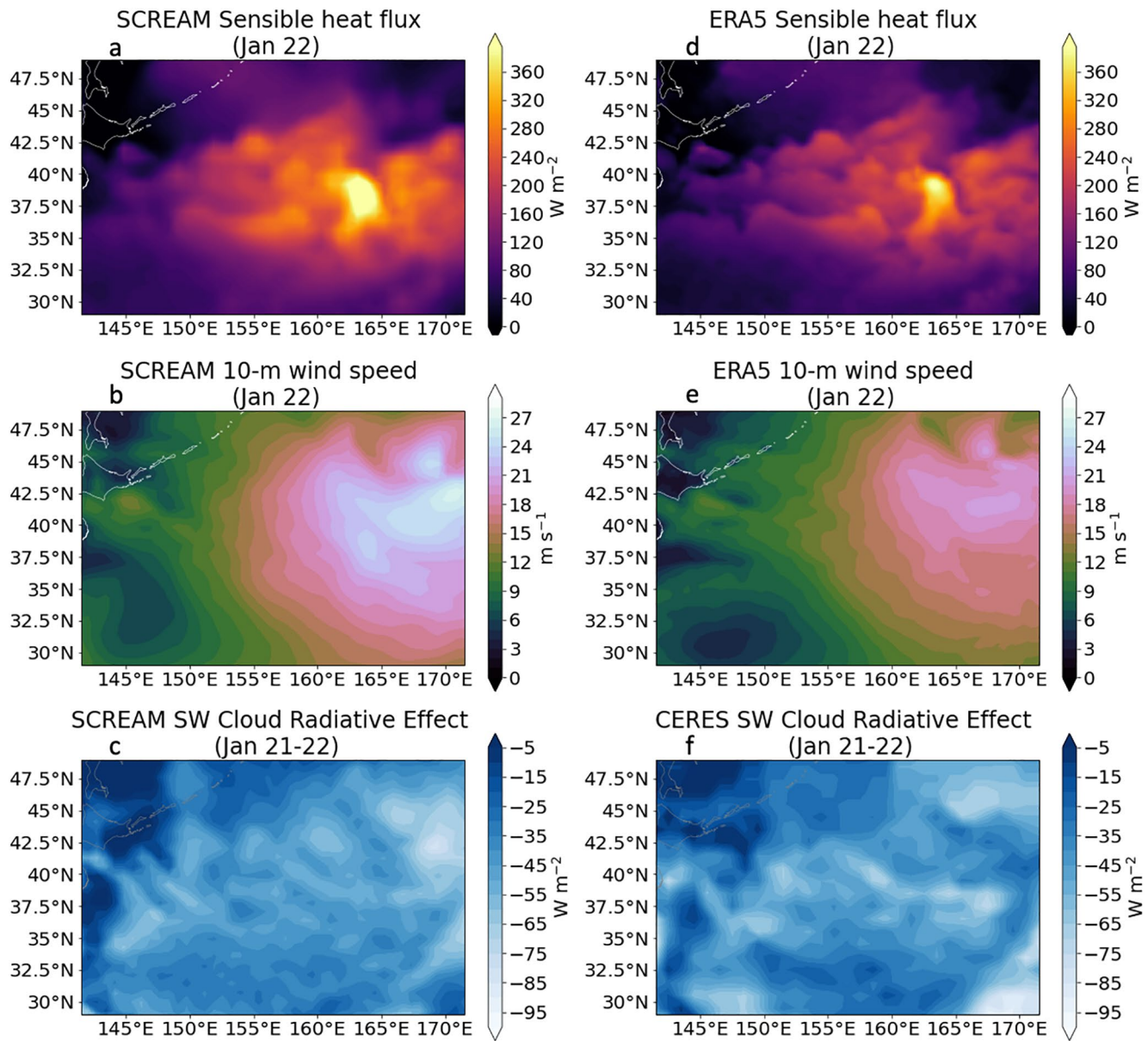
Figure 26. The daily mean sensible heat flux over the Kuroshio region bounded from 29° to 49°N and 141.5° to 171.5°E in SCREAM (a) and ERA5 (d) for the cold air outbreak on January 22. Also shown are similar daily mean values of 10-m wind speed (b) SCREAM; (e) ERA5 and shortwave cloud radiative effect (c) SCREAM; (f) CERES-SYN.
