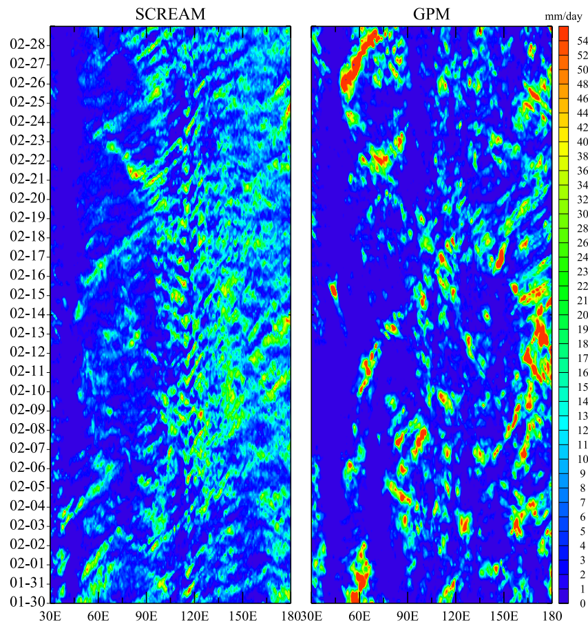
Figure 17. Precipitation averaged from 5°N to 5°S as a function of longitude (x-axis) and time (y axis) from SCREAM (left) and GPM precipitation observations (right).
