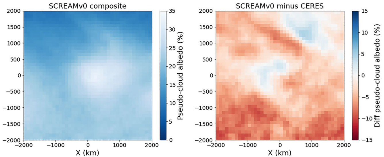
Figure 22. (left) Composite of the pseudo-cloud albedo in extratropical cyclones found between 45° and 60°S in SCREAM (January 20–February 28). Composites average over all 6 hourly snapshots centered on identified ECs and are plotted such that north is oriented upward. (right) Difference in storm composite pseudo-cloud albedo between storms in SCREAM and in reanalysis and satellite data (ERA5/CERES-SYN) for storms occurring during the same period.
