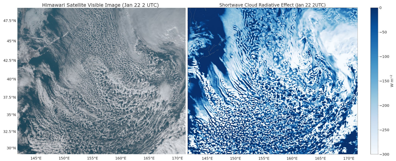
Figure 27. Cold-air outbreak off Siberia on January 22, 2020 at 2:00:00 UTC (~local noon) from a Himawari visible satellite image (left) and shortwave cloud radiative effect from SCREAM (right). Visualization is over a region bounded by 29°–49°N and 141.5° to 171.5°E.
