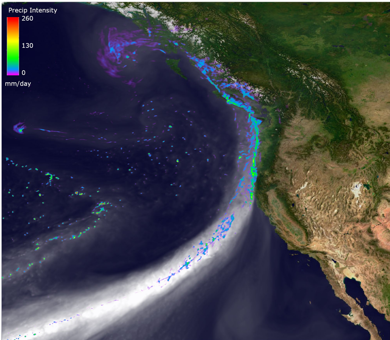
Figure 23. Snapshot of a landfalling atmospheric river along the west coast of North America that occurs on February 11, 23:00:00 UTC. Vertically integrated water vapor is indicated in transparent grayscale with opaque/white regions having integrated vapor greater than 40 \text{ kg m}^{-2} . Colors indicate precipitation intensity.
