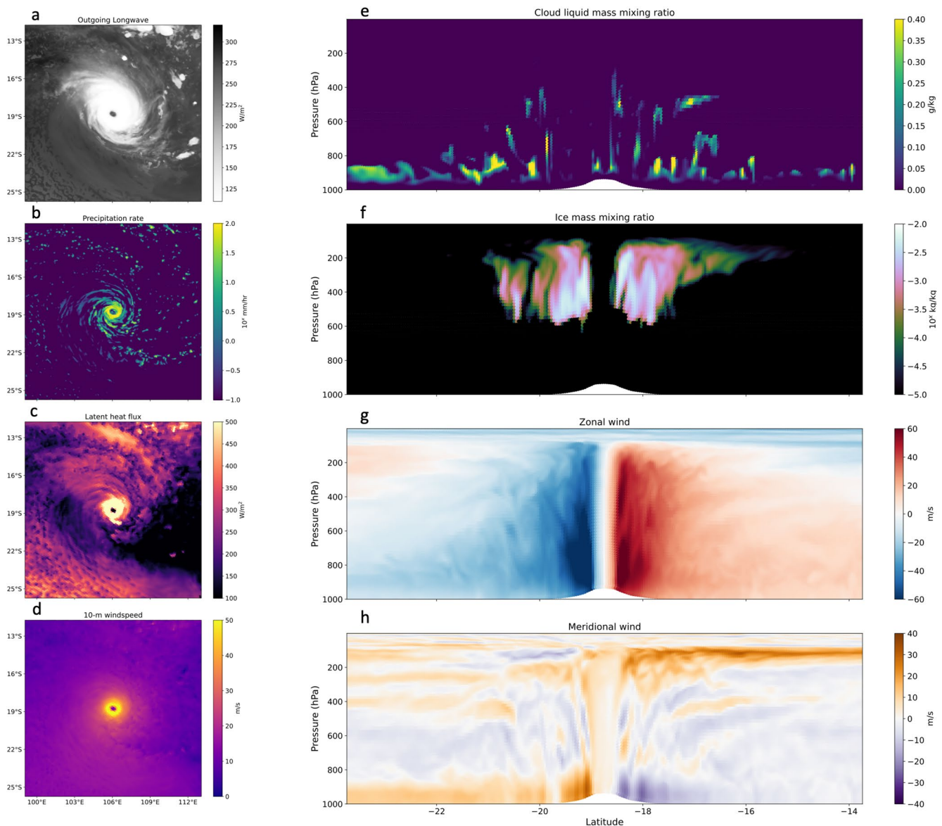
Figure 20. Instantaneous planar and curtain view of February 11 tropical cyclone at maximum intensity on February 16 0 UTC. On the left column are planar views of the (a) outgoing longwave radiation, (b) precipitation rate, (c) latent heat flux, and (d) 10-m wind speed. On the right column is a north-south curtain snapshot through the center of the storm of the (e) cloud liquid mass mixing ratio, (f) ice mass mixing ratio, (g) zonal wind speed, and (h) meridional wind speed.
