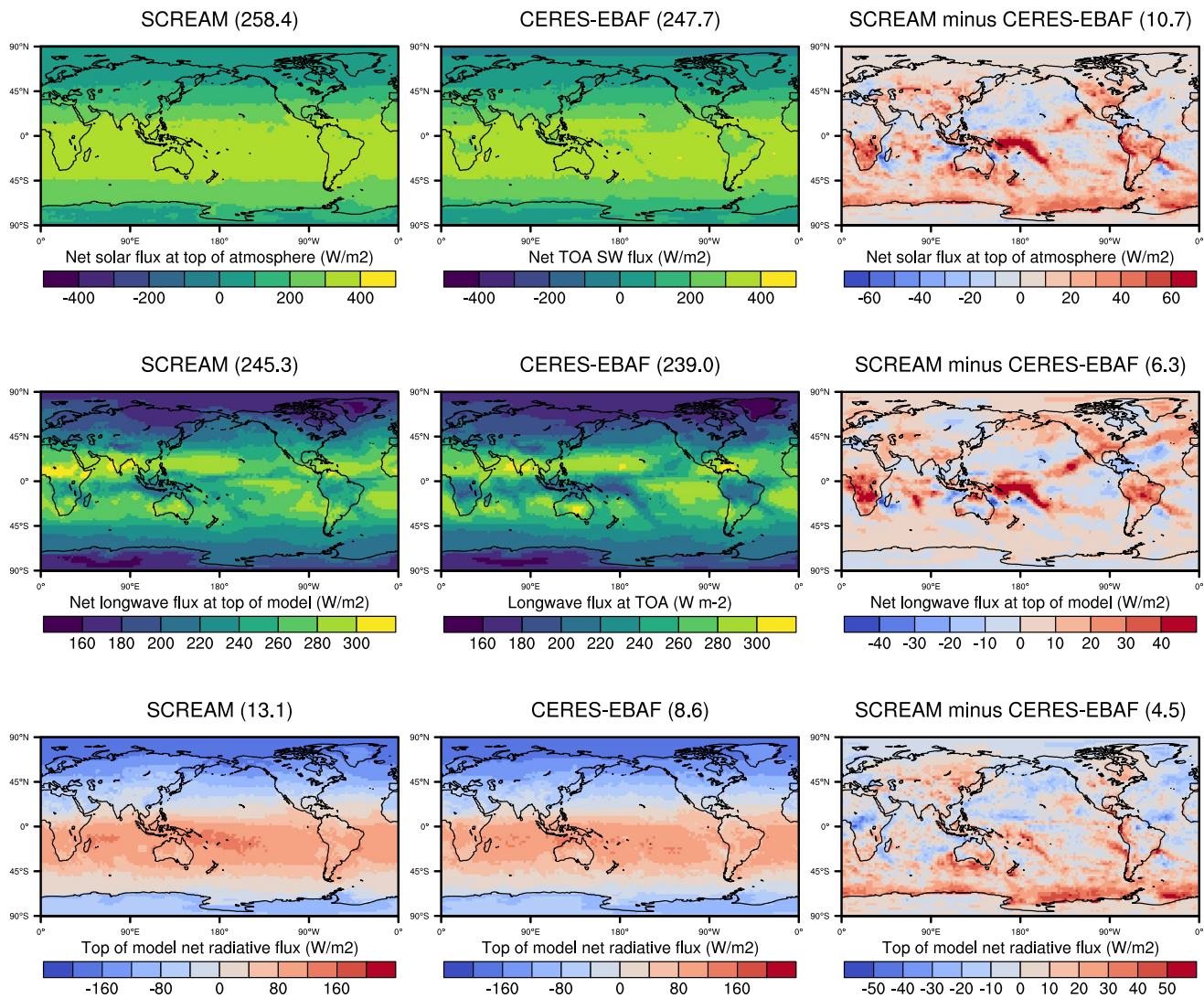
Figure 9. TOA radiation averaged over February 2020. Top is SW (>0 warms the planet), middle is LW (>0 cools the planet), and bottom is net (>0 warms the planet).
