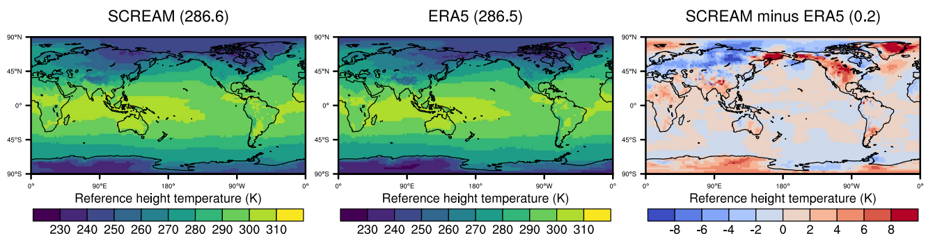
Figure 6. Near-surface temperature averaged over January 30 through February 28, 2020 from SCREAM and ERA5 reanalysis.
