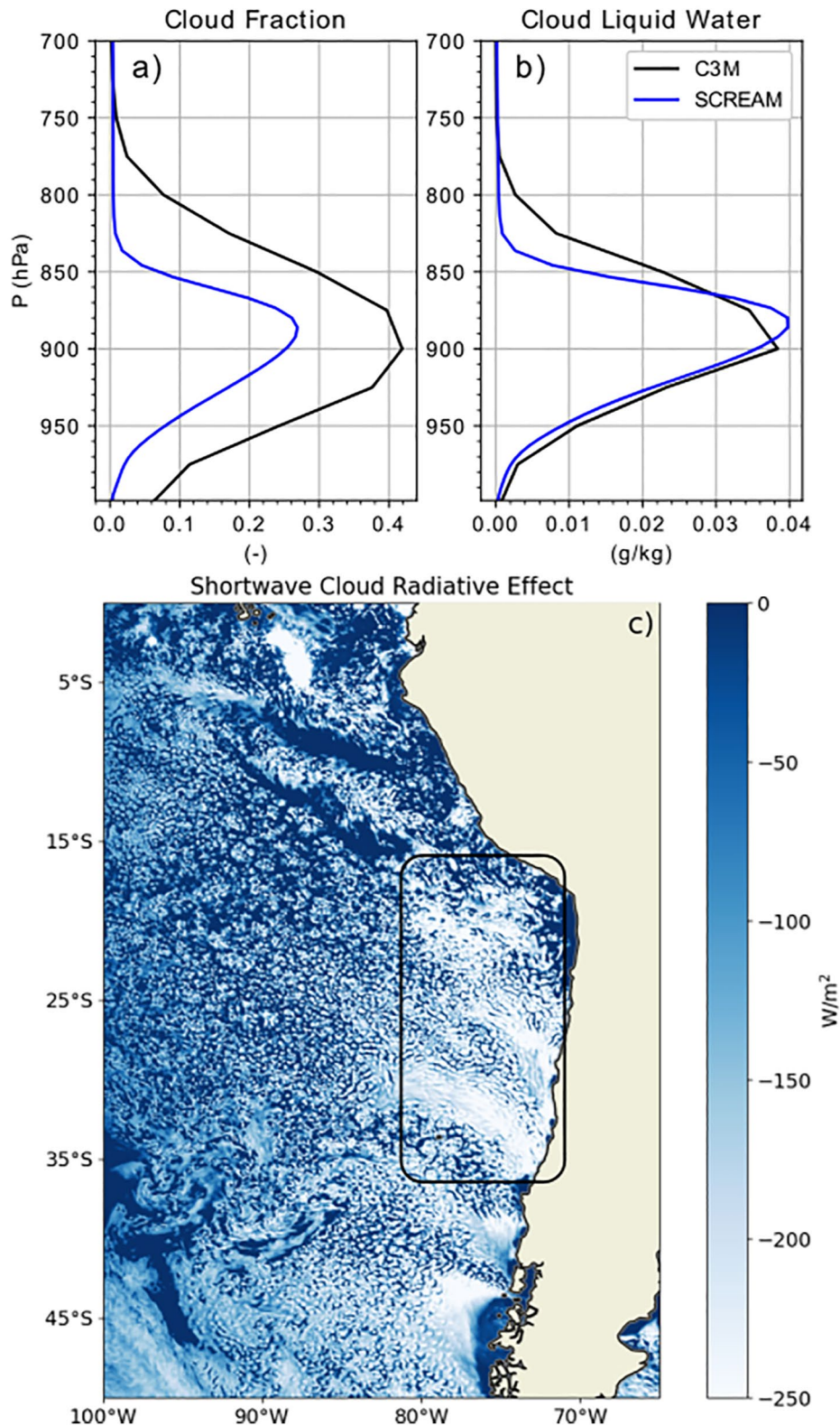
Figure 11. Temporally and spatially averaged profiles of (a) cloud fraction and (b) cloud liquid water for SCREAM and C3M. SCREAM profiles are averaged for the month of February 2020 while the C3M represents the February climatology from 2006 to 2010. Both SCREAM and C3M profiles represent spatial averages from the southeast Pacific coastal stratocumulus region bounded from 35° to 15°S and 275° to 290°E. The area used for spatial averaging is denoted in (c), which represents a snapshot of shortwave cloud radiative effect from SCREAM for March 1, 2020 at 18:00:00 UTC.
