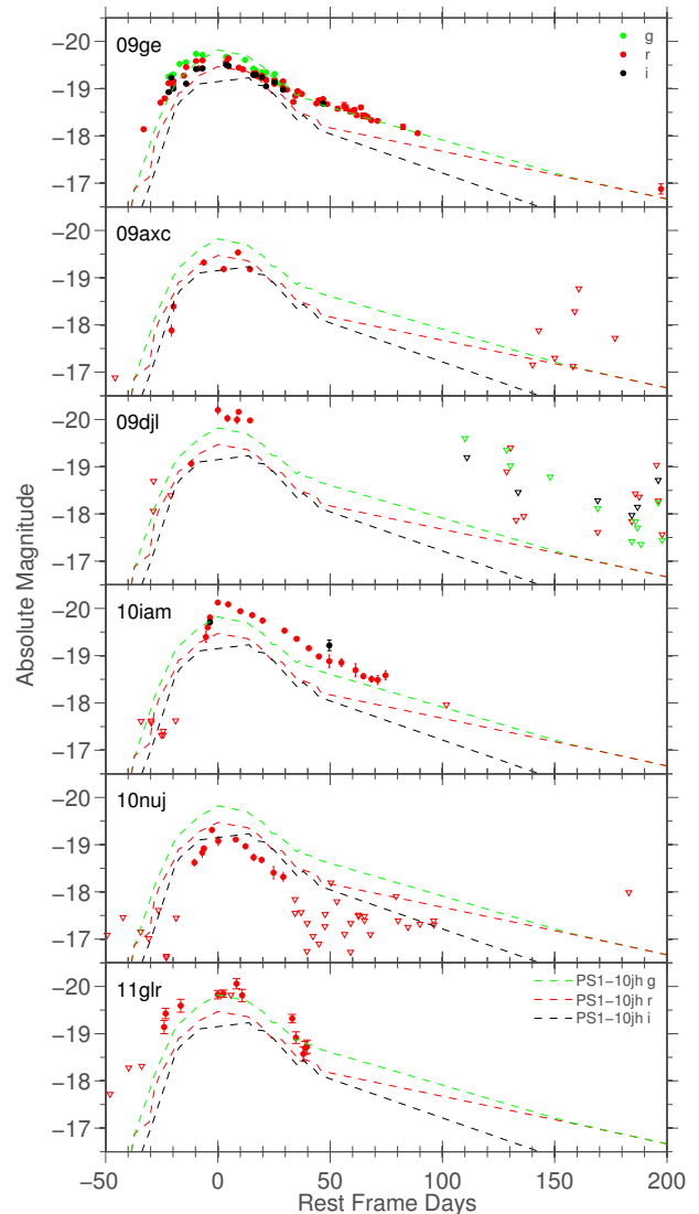
Figure 3. Light curves of PTF09ge, PTF09axc, PTF09djl, PTF10iam, PTF10nuj and PTF11glr from P48 and P60. Most display light curve shapes consistent with those of PS1-10jh (G12; dashed lines). PTF10iam shows a uniquely fast rise to peak, and PTF10nuj shows a sudden luminosity drop \sim 30 days after peak.
