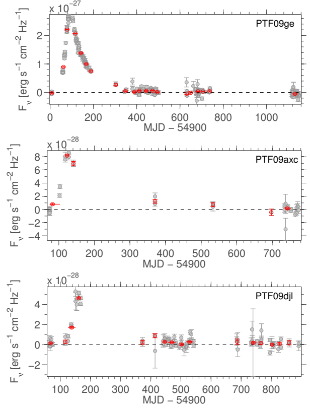
Figure 10. Long term host-subtracted R -band P48 light curves showing no subsequent activity at the locations of PTF09ge, PTF09axc and PTF09djl for a few hundred days after the original outburst (grey: raw data; red: 30-day binned data).
