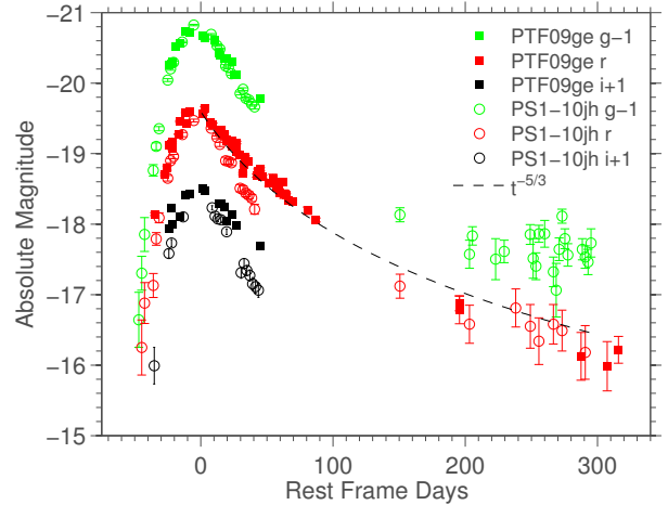
Figure 11. The g , r and i -band light curves of PTF09ge from P48 and P60, compared to those of PS1-10jh (G12). Both events show very similar photometric behavior. A t^{-5/3} decline rate is also shown.
