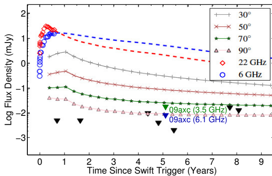
Figure 19. Radio non-detection limits of PTF09axc, 5 years after the eruption, over-plotted on Figure 1 from van Velzen et al. (2013). The open symbols show the observed radio light curve of Swift J1644+57. The dashed lines are predicted light curves from Berger et al. (2012) assuming a jet energy of 10^{52} erg. The van Velzen et al. (2013) 5 GHz off-axis light curve predictions are also shown. The triangles denote 2\sigma upper limits on the radio flux of the van Velzen et al. (2013) sample (black) and our data (green and blue). All data and models are scaled to the redshift of Swift J1644+57 ( z = 0.354 ). An off-axis jet is very unlikely for PTF09axc.
