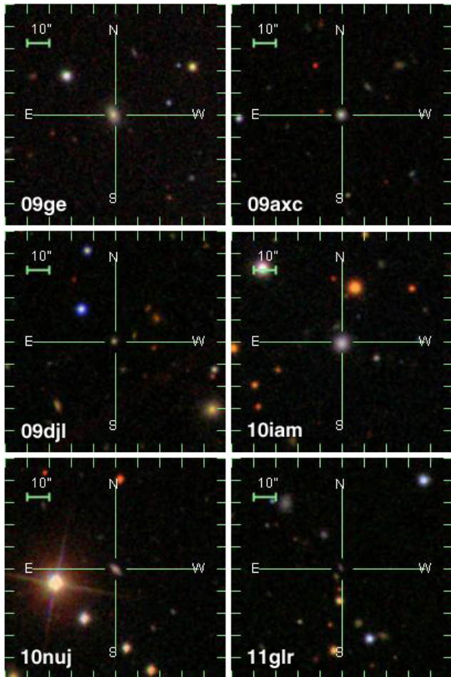
Figure 2. SDSS DR10 images centered at the locations of the events listed in Table 1.
