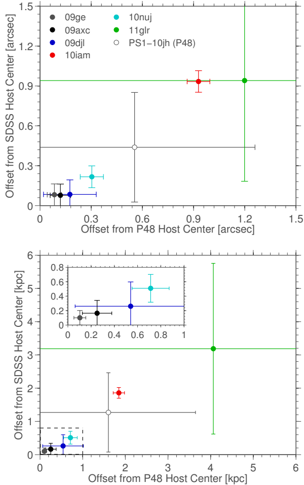
Figure 5. Offsets in arcseconds (top) and kpc (bottom) between the locations of our events and the centers of their hosts, determined both from P48 and from SDSS images of the hosts registered to P48 images of the transients. Error bars denote 1\sigma uncertainties. The region enclosed in the dashed box in the bottom panel is shown in greater detail in the inset. Three events (PTF09ge, PTF09axc and PTF09djl) are found to be coincident with the centers of their hosts with relatively small errors, one event (PTF10iam) is found to be offset from its host center, and for the remaining two events (PTF10nuj and PTF11glr) it is not possible to determine either an offset nor a robust coincidence with the center. The position of PS1-10jh (from its P48 detection as PTF10onn) is shown for comparison.
