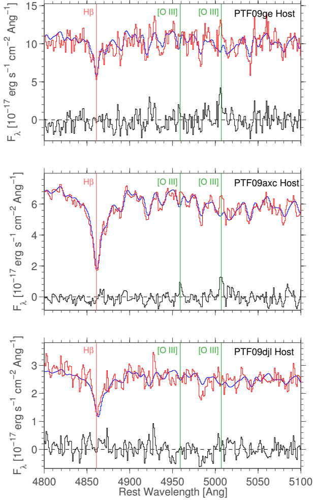
Figure 9. Host spectra (red), fitted stellar spectral templates (blue) and residuals (black). The spectra and templates are shifted in flux for clarity. PTF09axc shows an [OIII] 5007 Å emission line in the residual spectrum, marginally consistent with a weak AGN.
