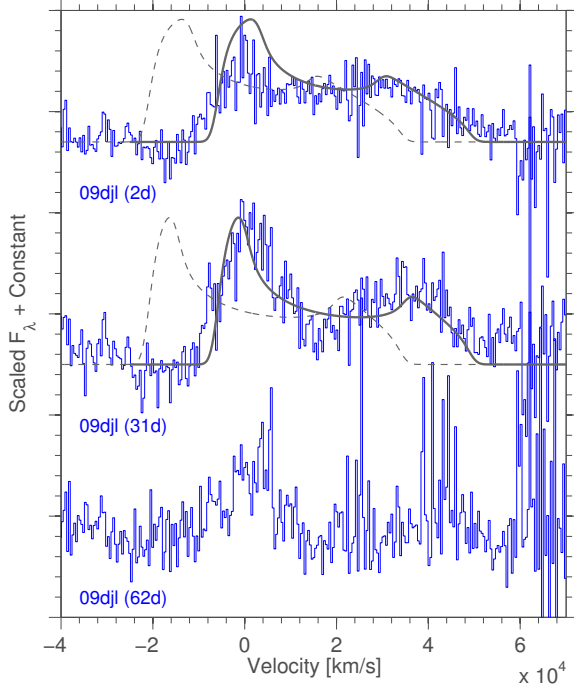
Figure 18. The H\alpha profile in the spectra of PTF09dj1 after host and continuum subtraction, corrected to the host redshift determined by its narrow absorption features. The data are binned to improve signal to noise, and phases are shown relative to peak. A red tail (first spectrum) and distinct red component (second spectrum) can be seen. A circular Keplerian disk model, following Strateva et al. (2003), is shown for inner and outer radii of 70 and 300 Schwarzschild radii (first spectrum) and 70 and 170 Schwarzschild radii (second spectrum), respectively. Both models assume an emissivity index of -3 , a local turbulent broadening of 1200 \text{ km s}^{-1} and an inclination angle of 50 degrees. The models are shifted to the red by 15000 \text{ km s}^{-1} (solid lines) from their original position (dashed lines).
