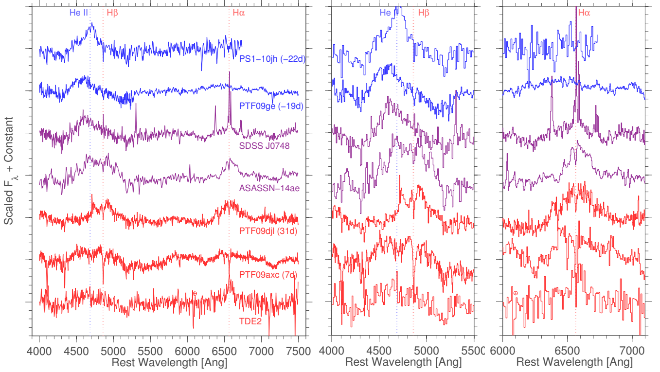
Figure 14. Continuum-subtracted spectra of our three PTF TDE candidates together with PS1-10jh (G12), ASASSN-14ae, SDSS J0748 (Wang et al. 2011) and TDE2 (van Velzen et al. 2011). Phases are shown relative to peak. A progression from He-rich to H-rich events is apparent. The middle and right panels present more detailed views of the regions around the marked lines.
