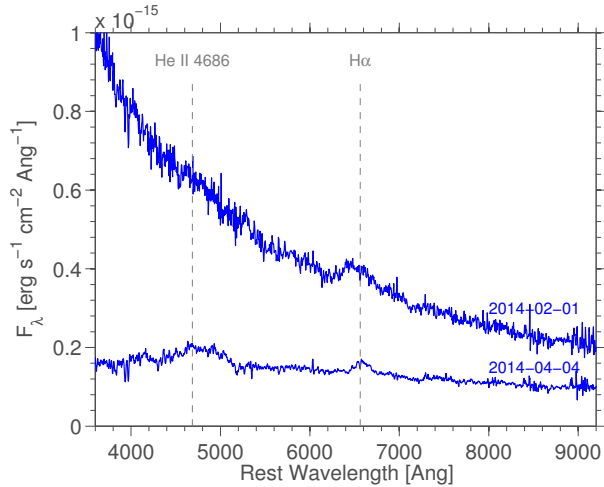
Figure 13. Spectra of ASASSN-14ae. The early spectrum displays broad H \alpha on top of a blue continuum. An additional broad component at He II 4686 Å appears in the later (cooler) spectrum.
