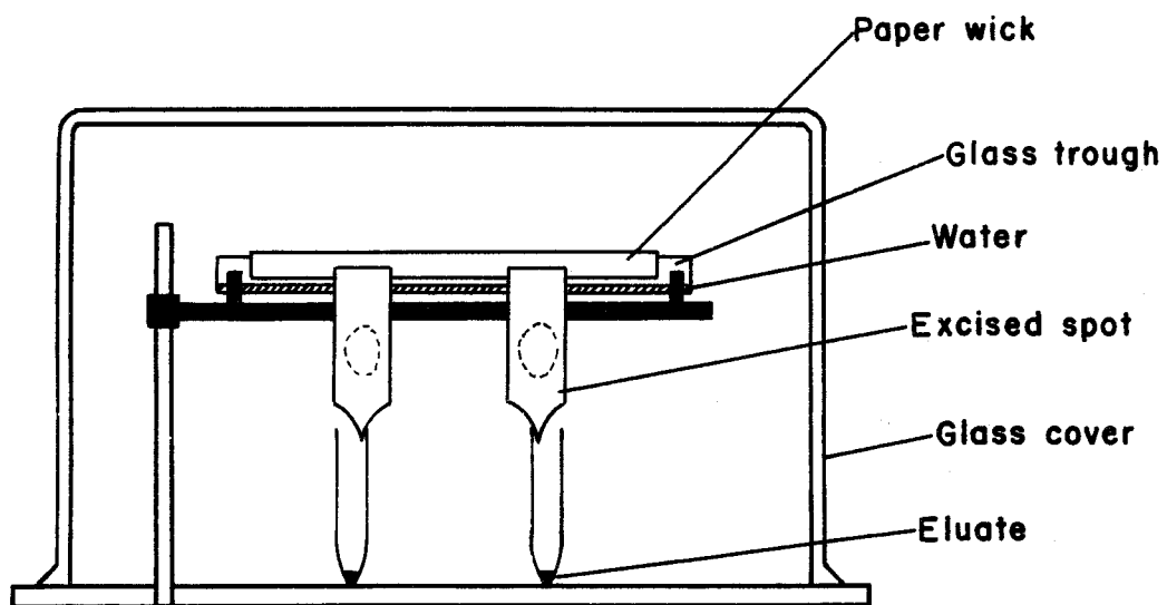
ELUTION APPARATUS FOR CHROMATOGRAPHED COMPOUNDS
