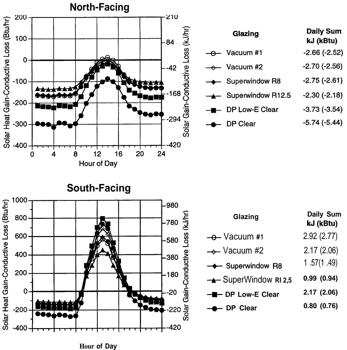
Figure 4: Window solar heat gain less conductive heat loss during a 24 hour period in January in Madison, Wi for a single-story residential house with a floor area of 143.1 m 2 (1540 ft 2 ) as a function of window type. Results are shown for 0.91 m x 1.21 m (3ft x 4ft) north- and south-facing windows.
