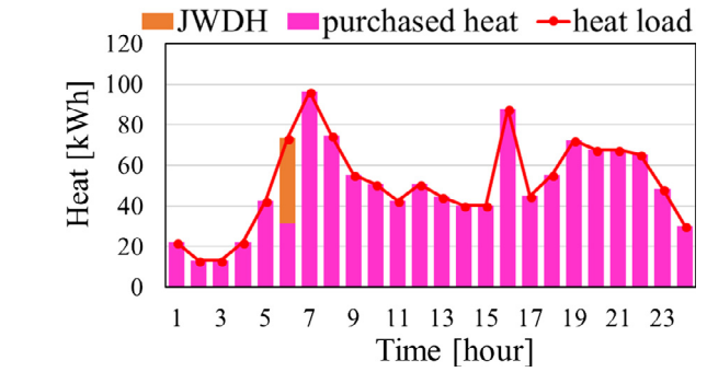
Fig. 10. Heat balance of the CEU model during a typical day 2 of Case A.
