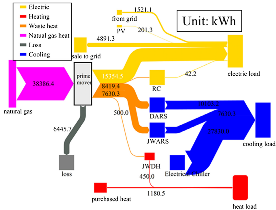
Fig. 5. Energy flow diagram for a summer (cooling) day in Case A.
