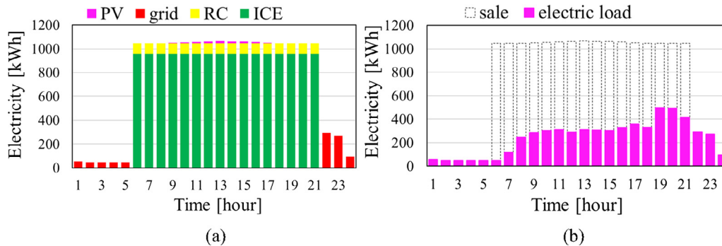
Fig. 6. Electricity balance in the CEU model during a typical day 1 of Case A (a. supply, b. demand).
