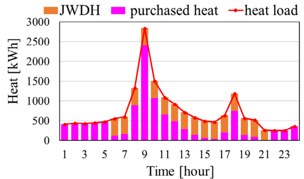
Fig. 7. Heat balance in the CEU model during a typical day 1 of Case A.
