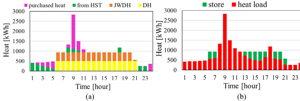
Fig. 22. Heat balance during a typical day 1 in Case D (a. supply, b. demand).
