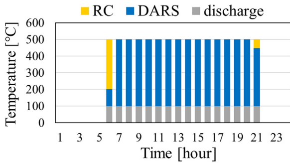
Fig. 12. Exhaust energy distribution during typical day 2 of Case A.
