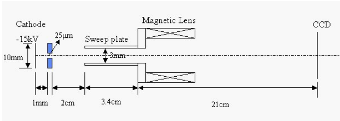
Figure 1: A schematic plot of the streak camera layout at ALS.
