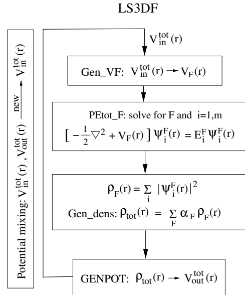
Fig. 2. LS3DF flow chart.
