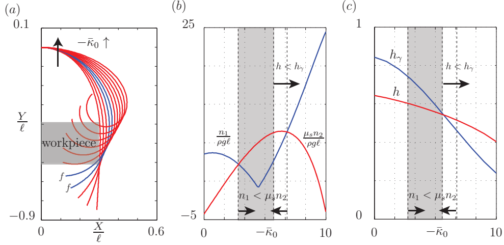
Figure 9: Grip III of the soft hand holding a given workpiece. (a) The deformed shape of the soft hand as \bar{\kappa}_0 varies with the pair of feasible configurations labelled f . (b) The corresponding dimensionless friction force \frac{n_1}{\rho g \ell} needed and the maximum friction force \frac{\mu_s n_2}{\rho g \ell} that can be provided. (c) The heights h and h_\gamma . The shaded regions in (b) and (c) are the feasible regions for Grip III. For the results shown, \frac{\gamma}{\ell} = 0.8 , \frac{b}{\ell} = 0.6 , D = \frac{EI}{\rho g \ell^3} = 1 , \mu_s = 1 , M = 5 , and -\bar{\kappa}_0 increases from 0 to 10.
