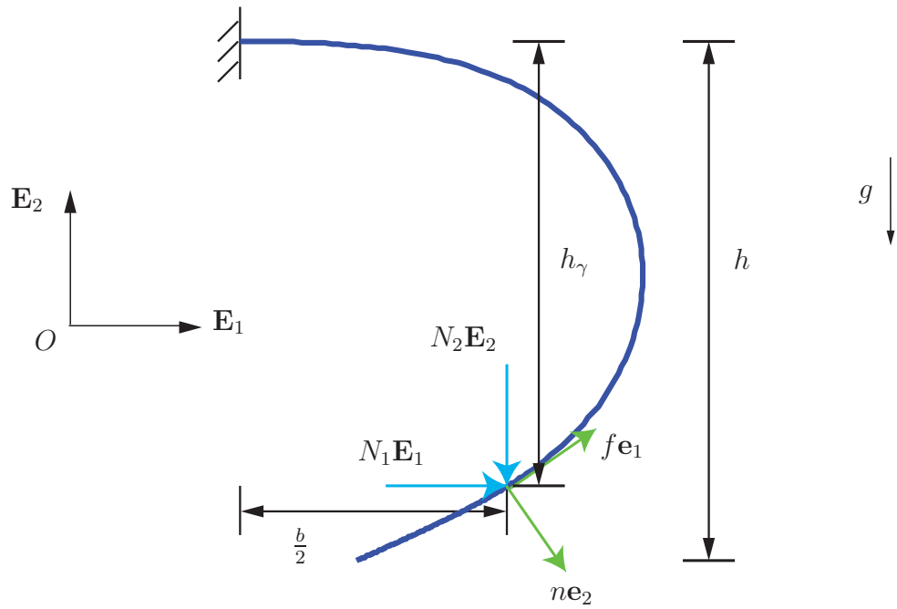
Figure 5: Schematic of the model for Grip III. Here, point contact of the workpiece and the rod occurs at the point s = \gamma . The workpiece is assumed to be held stationary by a normal force n\mathbf{e}_2 along with a static friction force f\mathbf{e}_1 . For the case shown, N_2 < 0 and f < 0 .
