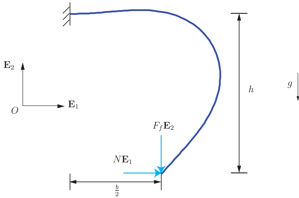
Figure 4: Schematic of the model for Grip I. In this model, the workpiece is assumed to be held stationary by static friction at the point contact at the tip of the rod s = \ell : \mathbf{F}_\ell = N\mathbf{E}_1 + F_f\mathbf{E}_2 .
