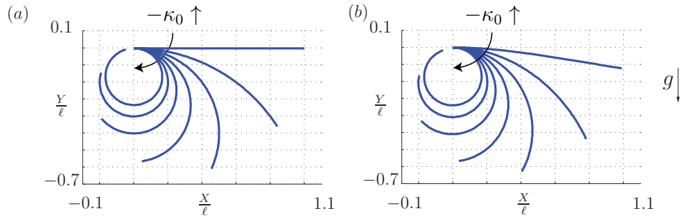
Figure 6: Features of the constant intrinsic curvature profile of a clamped-free rod as the constant \kappa_0 is varied. (a) The corresponding deformed shape of a rod with a constant intrinsic curvature profile. (b) The corresponding deformed shape of a heavy rod with a constant intrinsic curvature profile and a vertical gravity loading. The dimensionless flexural rigidity D of the rod is D = \frac{EI}{\rho g \ell^3} = 1 .
