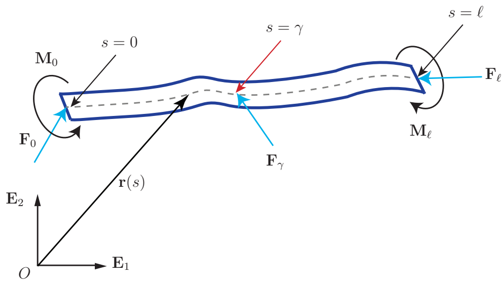
Figure 3: Schematic representation of an elastica of length \ell showing the position \mathbf{r} of a point on the centerline. The rod is subject to a terminal force \mathbf{F}_0 and terminal moment \mathbf{M}_0 at s=0 , a terminal force \mathbf{F}_\ell and terminal moment \mathbf{M}_\ell at the end s=\ell , and a force \mathbf{F}_\gamma at the point s=\gamma .
