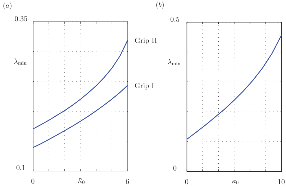
Figure 11: (a) Verification of the stability of the equilibrium configuration shown in Figures 7 and 8 by examining the minimum eigenvalue \lambda_{\min} of \mathbf{L} in an appropriate tangent subspace. (b) Verification of the stability of the equilibrium configuration shown in Figure 9 (i.e., Grip III); For the results shown, \frac{b}{\ell} = 0.6 , D = \frac{EI}{\rho g \ell^3} = 1 , M = 5 , and \mu_s = 1 .
