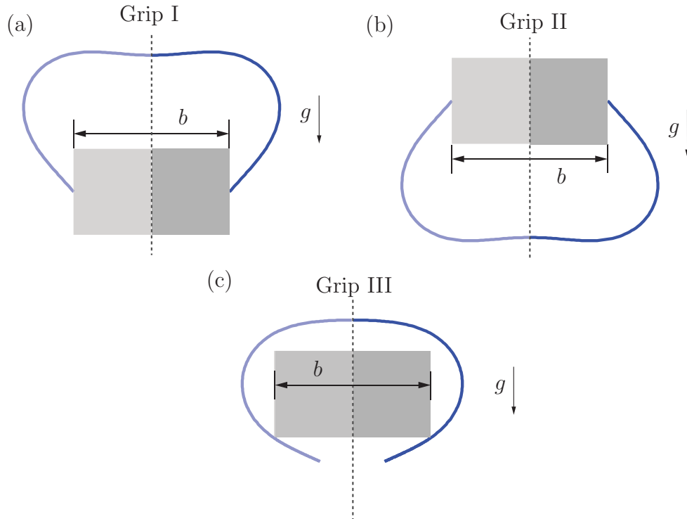
Figure 2: Illustration of three typical gripping modes of a workpiece with the width b . In Grips I & II which are shown in (a) and (b), respectively, the workpiece is lifted with the help of static friction forces at the tip of the finger. In Grip III, which is shown in (c), the workpiece is lifted by the normal (pinching) force together with static friction forces at the contact point of the finger with the workpiece.
