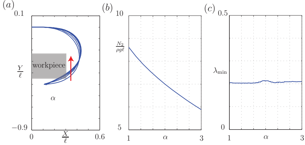
Figure 15: Grip III of the soft hand holding a given workpiece. (a) The deformed shape of the soft hand as \alpha varies. (b) The corresponding maximum force \frac{N_2}{\rho g \ell} that can be provided (i.e., the load bearing capacity). (c) Verification of the stability of the equilibrium configuration obtained by examining the minimum eigenvalue \lambda_{\min} of \mathbf{L} in an appropriate tangent subspace. For the results shown, \frac{b}{\ell} = 0.6 , D = \frac{EI}{\rho g \ell^3} = 1 , \mu_s = 1 , \bar{\kappa}_{max} = 6 , M = 5 , and \alpha increases from 1 to 3.
