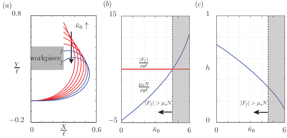
Figure 8: Grip II of the soft hand. (a) The deformed shape of the soft hand as \bar{\kappa}_0 varies with the pair of feasible configurations labelled with f . (b) The corresponding dimensionless friction \frac{|F_f|}{\rho g \ell} required and the maximum friction \frac{\mu_s N}{\rho g \ell} that can be provided. (c) The height h of the tip of the rod. The shaded regions in (b) and (c) indicates the feasible regions for Grip II . For the results shown, \frac{b}{\ell} = 0.6 , D = \frac{EI}{\rho g \ell^3} = 1 , \mu_s = 1 , M = 5 , and \bar{\kappa}_0 increases from 0 to 6.
