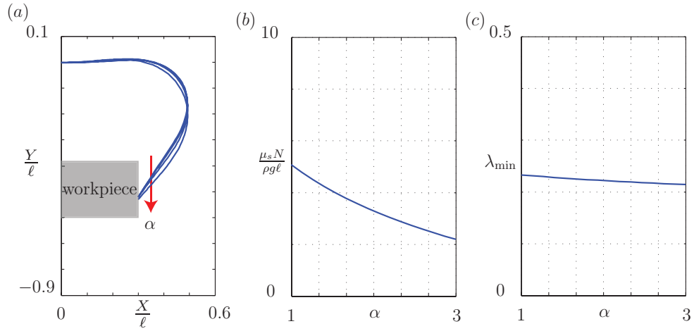
Figure 13: Grip I of the soft hand where the workpiece faces downwards. (a) The deformed shape of the soft hand as \alpha varies. (b) The corresponding maximum dimensionless friction force \frac{\mu_s N}{\rho g \ell} that can be provided, (i.e., the loading bearing capacity). (c) Verification of the stability of the equilibrium configuration obtained by examining the minimum eigenvalue \lambda_{\min} of \mathbb{L} in an appropriate tangent subspace. For the results shown, \frac{b}{\ell} = 0.6 , D = \frac{EI}{\rho g \ell^3} = 1 , \mu_s = 1 , \bar{\kappa}_{max} = 6 , M = 5 , and \alpha increases from 1 to 3.
