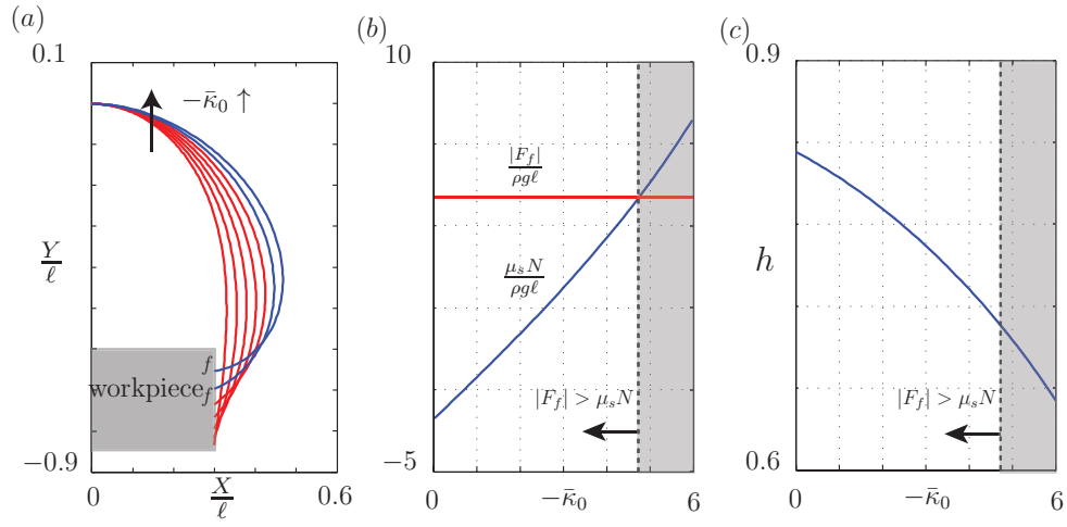
Figure 7: Grip I of the soft hand. (a) The deformed shape of the soft hand as \bar{\kappa}_0 varies with the pair of feasible configurations labelled f . (b) The corresponding dimensionless friction \frac{|F_f|}{\rho g \ell} required and the maximum friction \frac{\mu_s N}{\rho g \ell} that can be provided. (c) The height h of the tip of the rod. The shaded regions in (b) and (c) indicates the feasible regions for Grip I. For the results shown, \frac{b}{\ell} = 0.6 , D = \frac{EI}{\rho g \ell^3} = 1 , \mu_s = 1 , M = 5 and -\bar{\kappa}_0 increases from 0 to 6.
