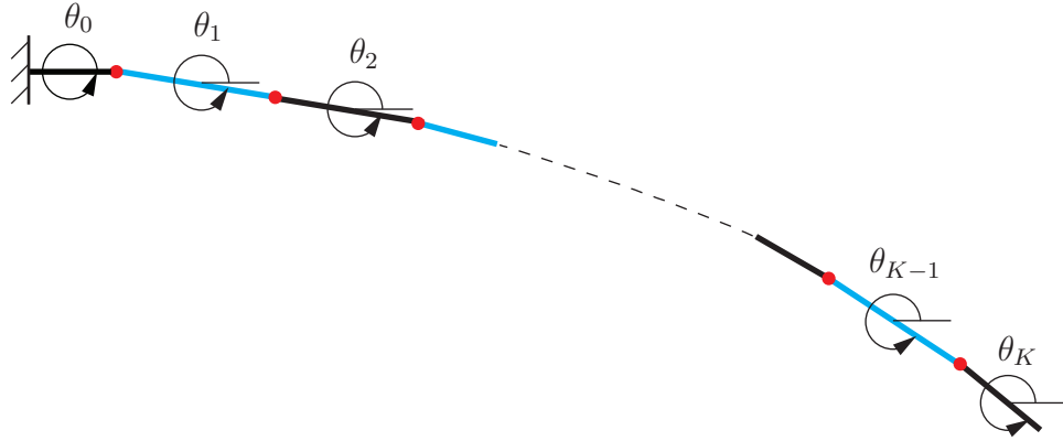
Figure 10: Schematic of the discretization scheme for the rod.
