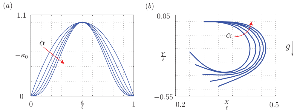
Figure 12: Features of the curvature profile given by (34) as the parameter \alpha is varied. (a) The dimensionless intrinsic curvature throughout the deformed rod. (b) The corresponding deformed shape of a heavy rod with an intrinsic curvature profile (34). For the results shown, \bar{\kappa}_{max} = 6 , p = -1 , and D = \frac{EI}{\rho g \ell^3} = 1 .
