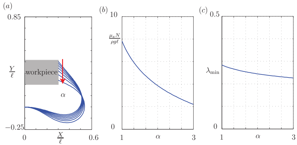
Figure 14: Grip II of the soft hand where the workpiece points upwards. (a) The deformed shape of the soft hand as \alpha varies. (b) The corresponding maximum dimensionless friction force \frac{\mu_s N}{\rho g \ell} that can be provided, (i.e., the loading bearing capacity). (c) Verification of the stability of the equilibrium configuration obtained by examining the minimum eigenvalue \lambda_{\min} of \mathbb{L} in an appropriate tangent subspace. For the results shown, \frac{b}{\ell} = 0.6 , D = \frac{EI}{\rho g \ell^3} = 1 , \mu_s = 1 , \bar{K}_{max} = 6 , M = 5 , and \alpha increases from 1 to 3.
