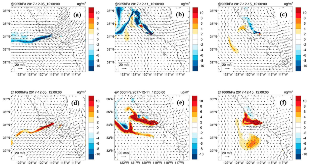
Figure 7. Distribution of PM 2.5 concentration difference between the V_VIIRS and V_VIIRS_Plus scenarios at 925 hPa (a–c) and 1,000 hPa (d–f) levels.
