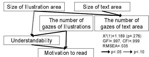
Figure 2: Result of structural equation modeling. Note that the non-significant effects ( p > .10 ) were removed from the figure.
