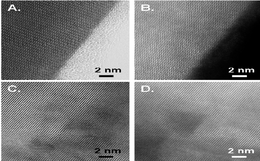
Figure 2. BF and HAADF HRSTEM images of as grown and annealed \text{In}_x\text{Ga}_{1-x}\text{N} nanowires. A comparison of (A) BF and (B) HAADF HRSTEM images from an \text{In}_x\text{Ga}_{1-x}\text{N} ( x = 0.28 ) nanowire shows that it is homogeneous in composition. After annealing at 800\text{ }^\circ\text{C} , (C) BF and (D) HAADF HRSTEM images show triangular indium depleted regions, indicating that samples become inhomogeneous.
