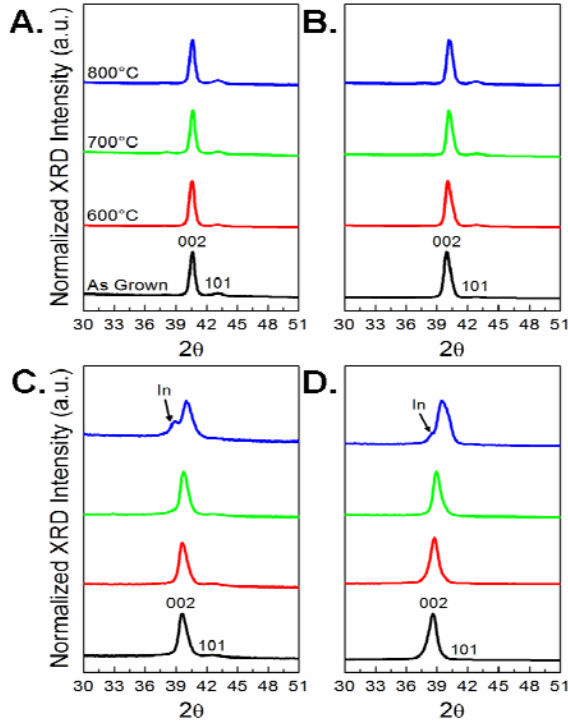
Figure 3. XRD spectra of as grown and annealed \text{In}_x\text{Ga}_{1-x}\text{N} nanowires. XRD spectra corresponding to samples (A) x = 0.07 , (B) x = 0.17 , (C) x = 0.28 , and (D) x = 0.42 showing the wurtzite 002 and 101 peaks of \text{In}_x\text{Ga}_{1-x}\text{N} nanowires after annealing at a series of temperatures. Diffraction peaks shift towards higher angles because of a decrease in lattice constant from the etching of indium. Higher indium composition samples (C,D) show an additional In 101 peak from the decomposition of InGaN.
