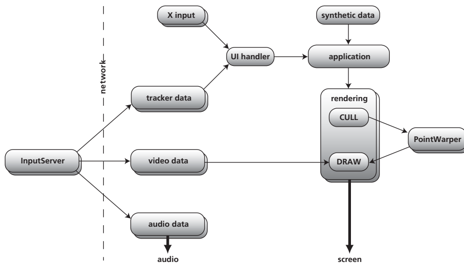
Figure 3: Dataflow of a typical JAPE application.
