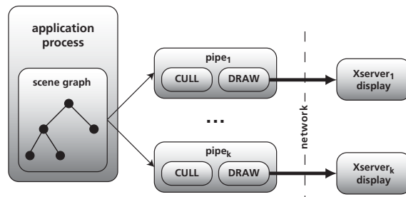
Figure 2: The multi-head rendering concept.
