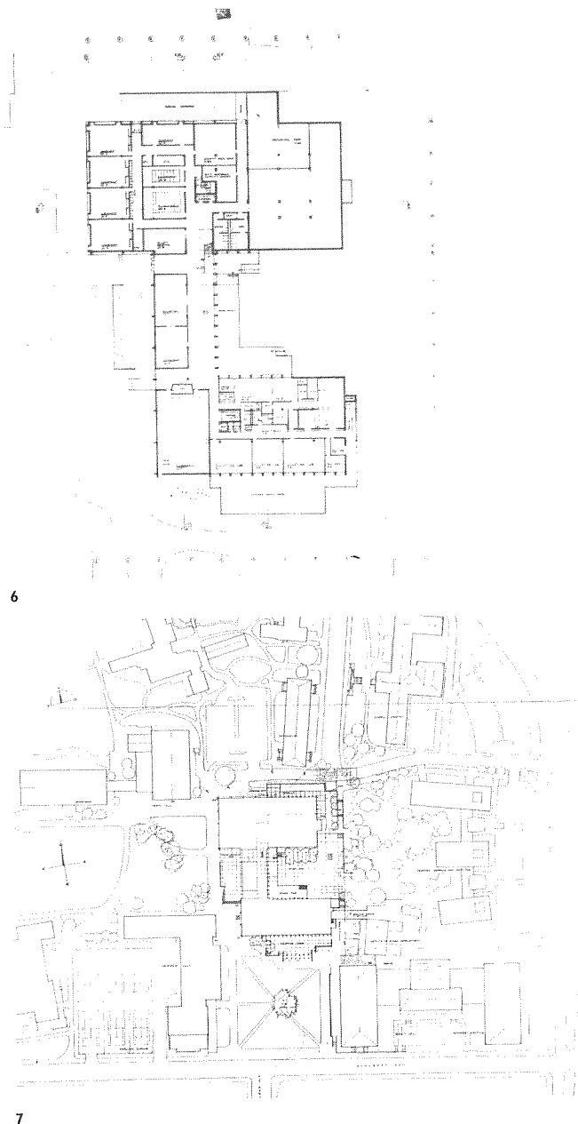
6 Ground floor plan of the November 1, 1960, scheme.
