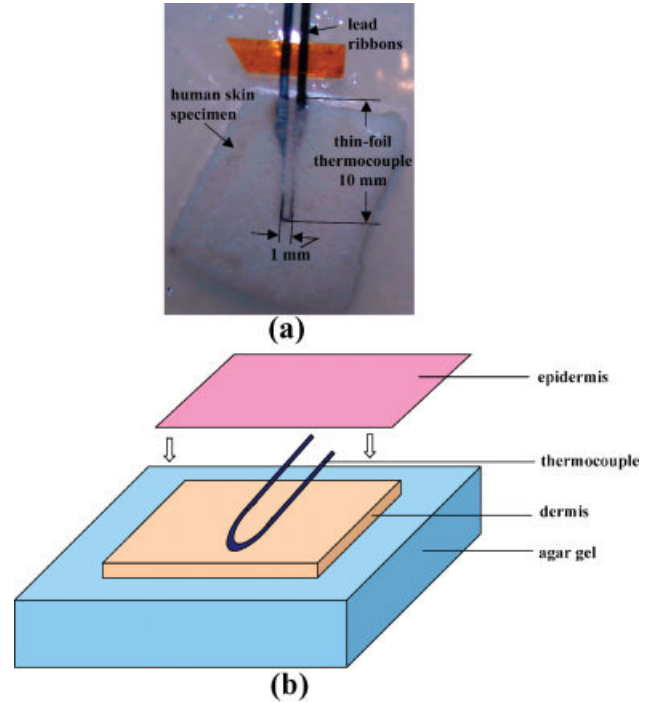
Fig. 1. Photo (a) and schematics (b) show how ex vivo human skin specimens were placed on top of an agar gel phantom. A thick type-K thin-foil thermocouple was inserted between the separated epidermis and dermis.
