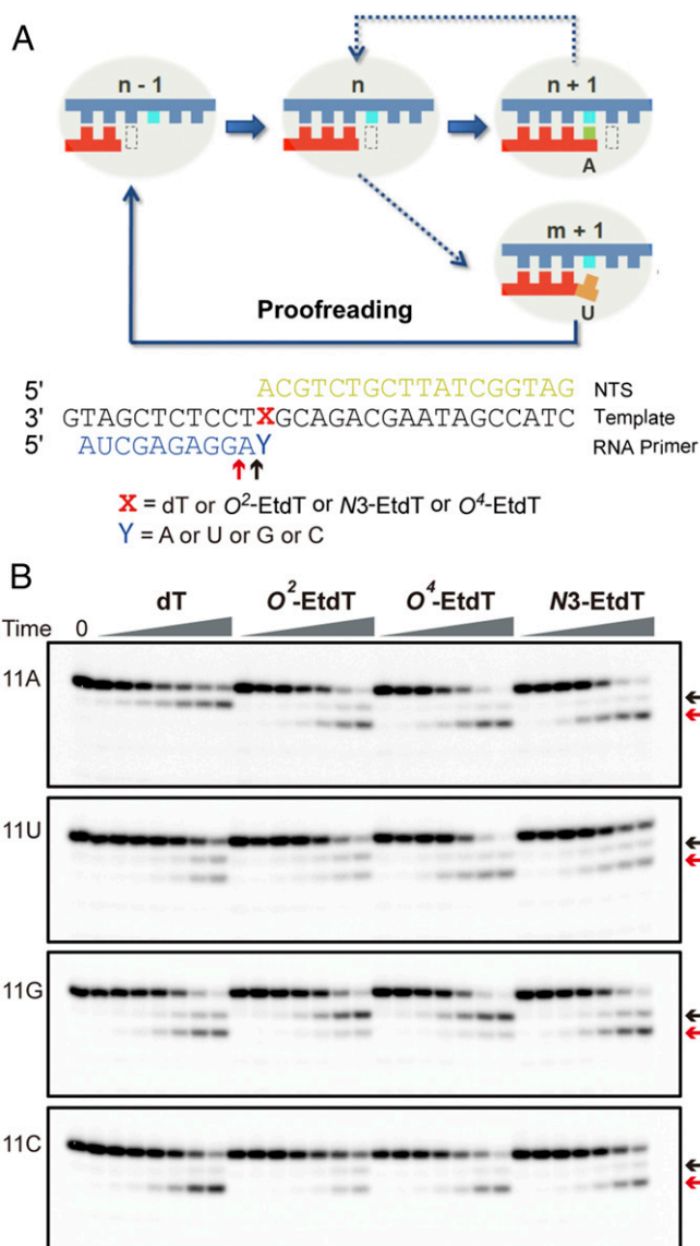
Fig. 4. Backtrack and proofreading of RNA pol II after nucleotide insertion opposite the ethylated thymidine lesions. (A) Scaffold used in the cleavage assay. (B) Results of RNA pol II intrinsic cleavage. The black arrow refers to the pretranslocation cleavage product; the red arrow refers to the backtrack cleavage product. The time points were 5 min, 20 min, 60 min, 3 h, 8 h, 24 h, and 48 h, respectively.
