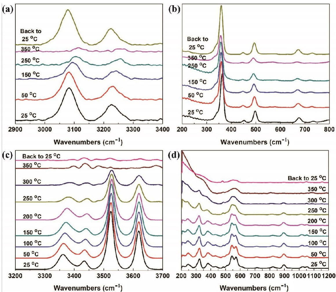
Figure 8. Temperature-dependent (25 to 350 °C) Raman spectra for (a) and (b) boehmite and (c) and (d) gibbsite.
