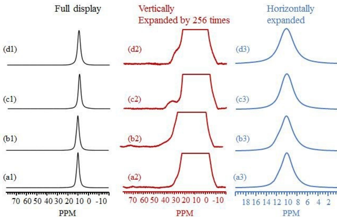
Figure 6. ^{27}Al MAS NMR spectra acquired on a 850 MHz NMR
