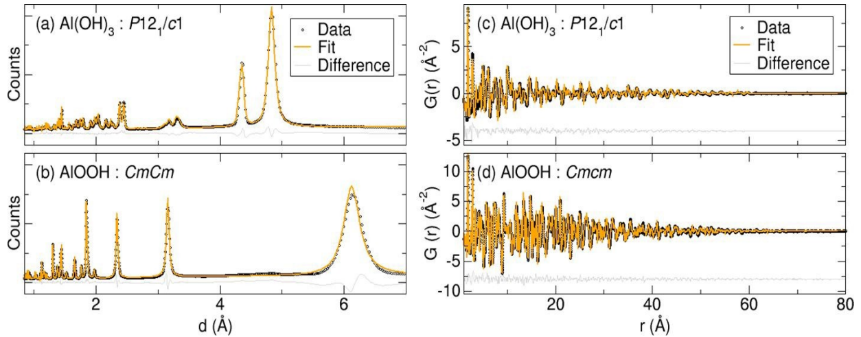
Figure 4. Results of Rietveld refinement of the (a) gibbsite and (b) boehmite nanoplates using X-ray diffraction data from 11-ID-B. First 80 Å of PDF fits of 1 to 100 Å (c) gibbsite and (d) boehmite nanoplate X-ray PDF data, resulting from models with an anisotropic particle shape function.
