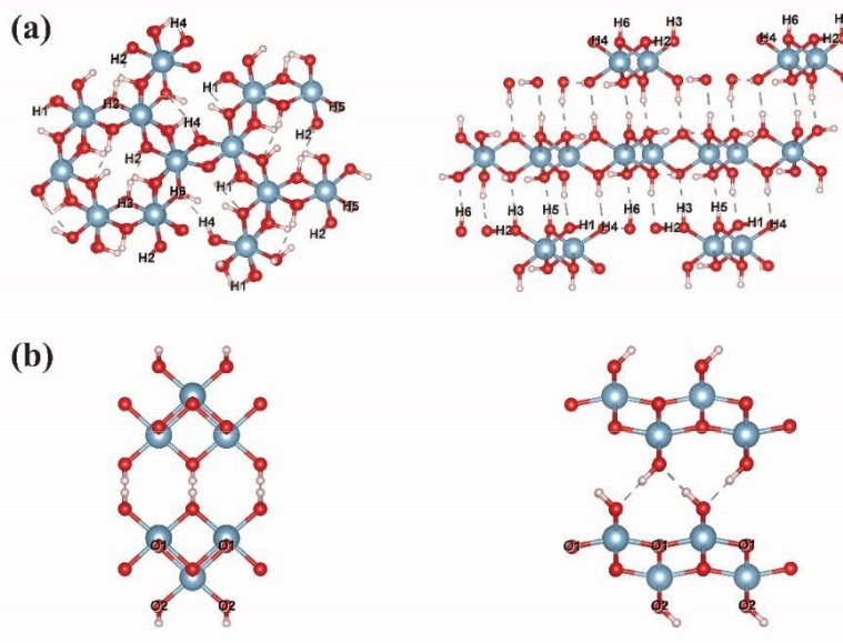
Figure 1. Crystal structure of gibbsite (a) and boehmite (b).
