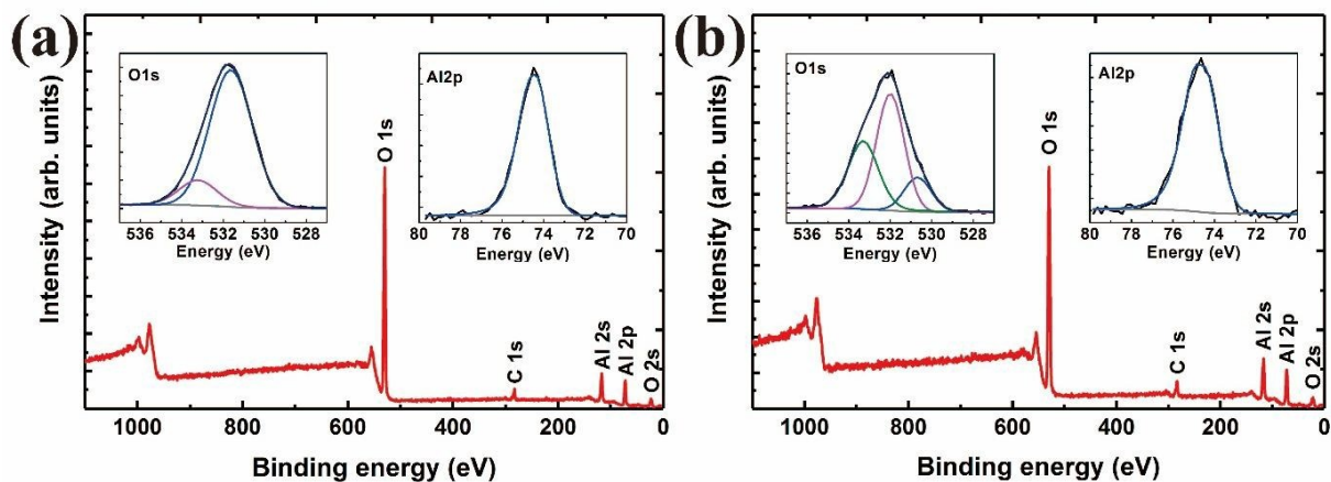
Figure 7. XPS survey scan of (a) gibbsite (b) boehmite with top inset : oxygen 1s high resolution scan and bottom inset : aluminum 2p high resolution scan.
