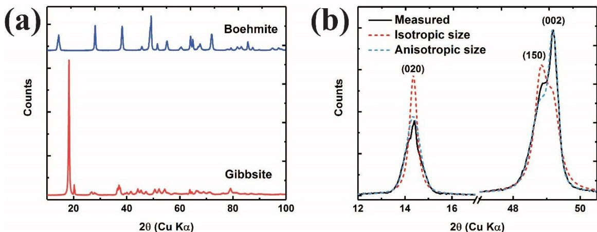
Figure 3. XRD patterns of gibbsite (lower in a) and boehmite (upper in a) nanoplates, and (b) detail of boehmite XRD pattern compared with simulated patterns incorporating either isotropic or anisotropic crystallite size broadening.
