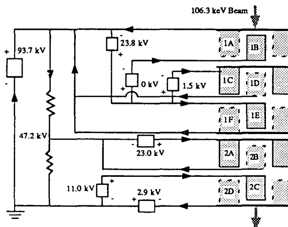
Fig. 2. Circuit diagram of the ESQ accelerator.
