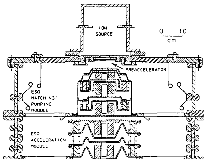
Fig. 1. Schematic Diagram of the prototype ESQ Accelerator
