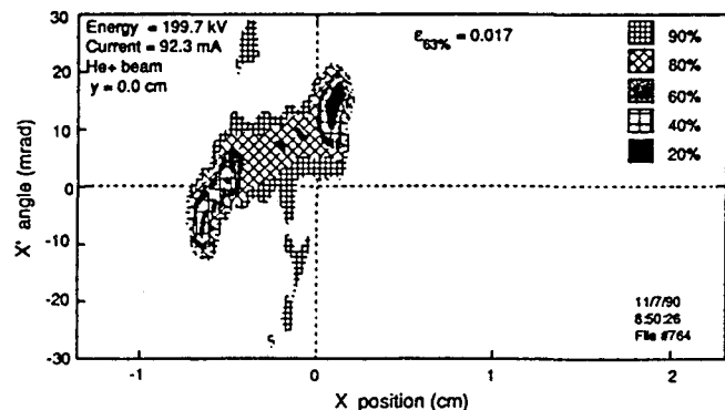
Fig. 4. Emittance Diagram of a 92.3 mA He^+ beam leaving the ESQ accelerator at 200 keV energy.
