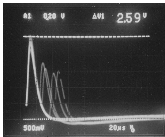
Fig. 7. Photograph of oscilloscope traces of pulses seen in LAr with 2500ppm Kr and 1400V applied to the drift electrode at ~ 1.3 atmospheres pressure (5psig). First (and largest) pulse is about 2.6V, and the pulse width of ~ 1μs fwhm is determined by the amplifier time constants.
