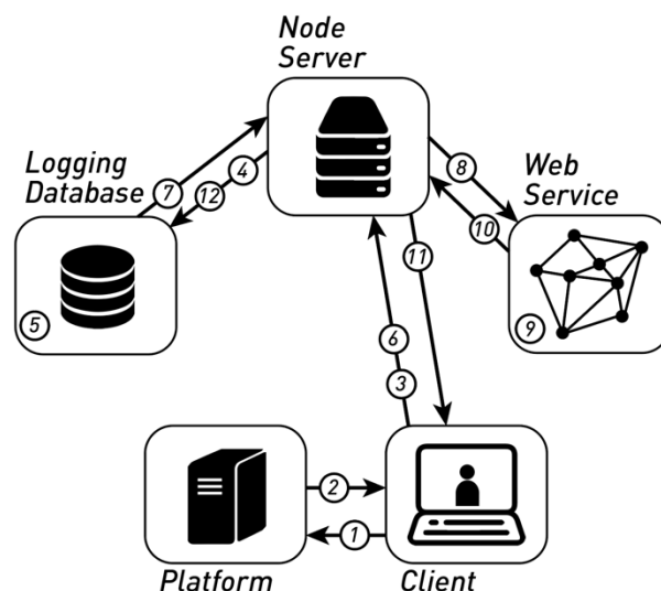
Figure 2. Diagram visualizing the entire process of delivering a recommendation to the learner. The circled numbers correspond to the numbered steps below.
