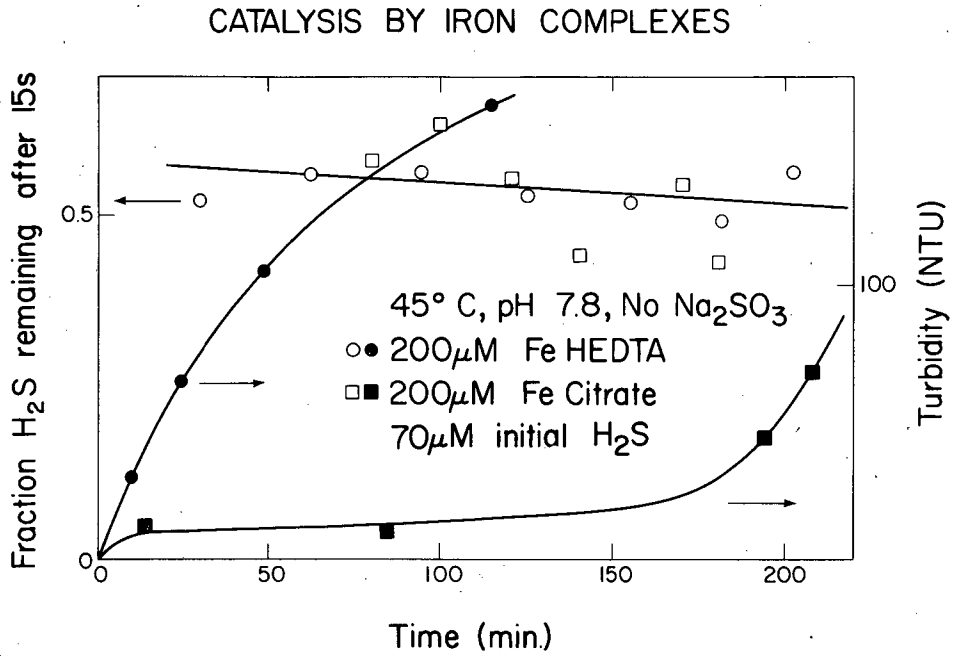
Fig. 4.5. Reaction catalyzed by iron complexes. Data generated by continuous recharge method, as with nickel. Difference in recorded turbidities may not be significant.
