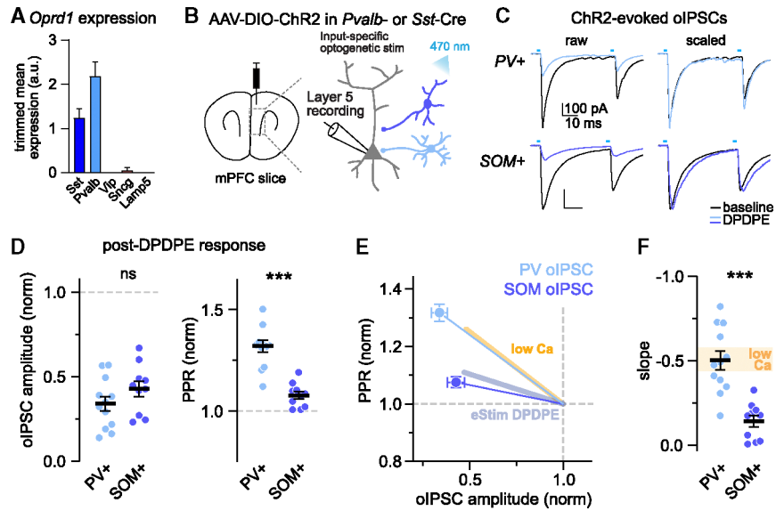
Figure 2. GABA release from PV+ and SOM+ interneurons is differentially regulated by DORs (A) Expression of Oprd1 mRNA across GABAergic cell classes from Allen Institute mouse patch-seq database. 43
