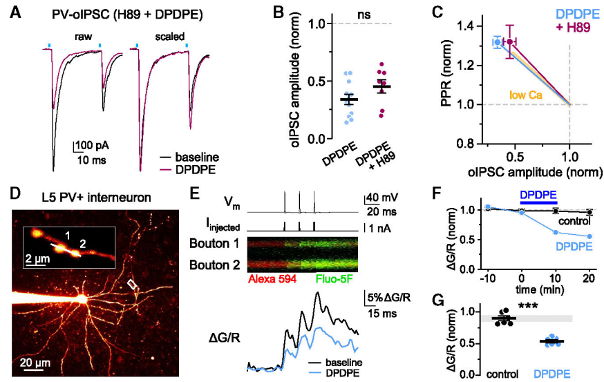
Figure 3. DORs mediate canonical Ca_v inhibition in PV+ interneurons
