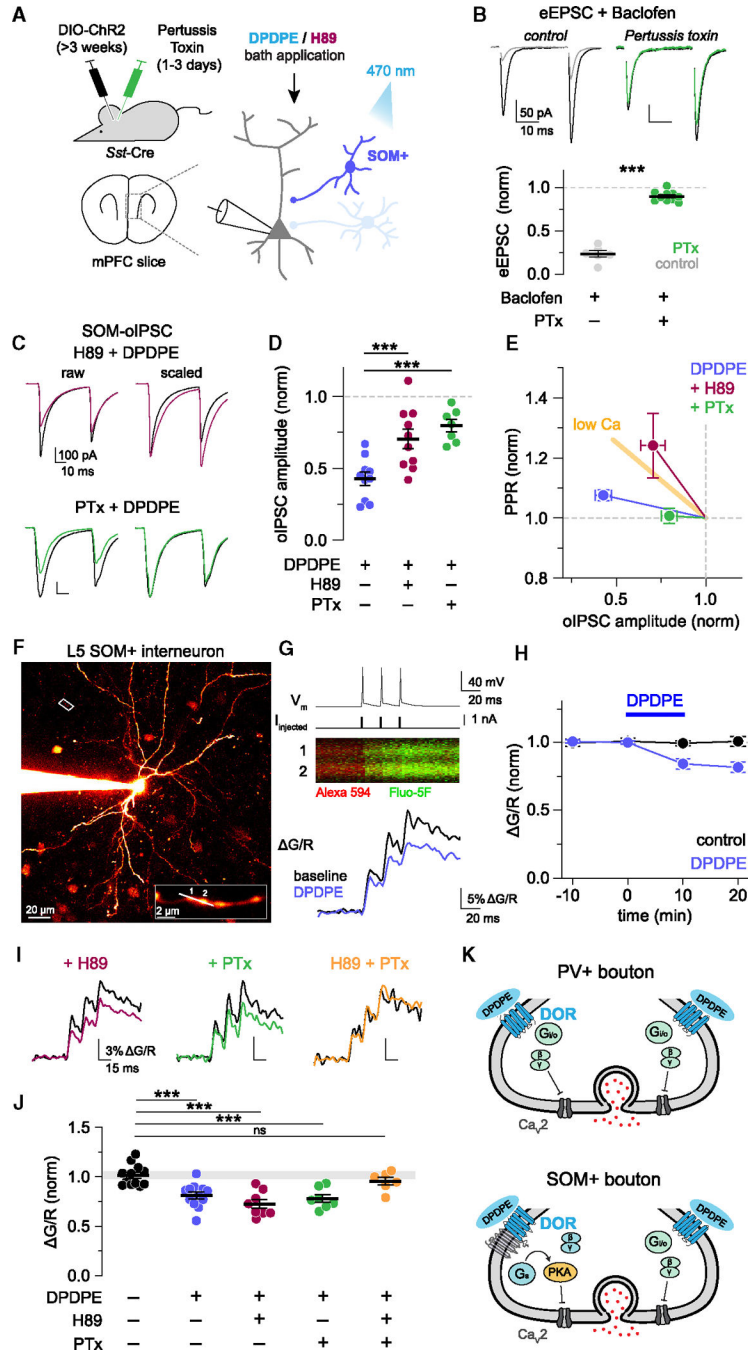
Figure 4. SOM+ interneurons exhibit heterogeneous regulation by DORs
