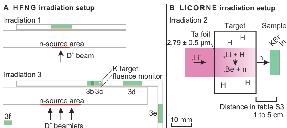
Fig. 4. Irradiation setup of neutron cross section experiments. (A) Geometry of samples in the HFNG with respect to the neutron source area where the \text{D}^+ beamlets impinge on the Ti layer hosting the interstitially implanted D. The neutron energy spectrum each target was exposed to is given in Fig. 5). (B) Setup of the LICORNE experiment and irradiation geometry. Table 1 and table S3 list the irradiation details.
