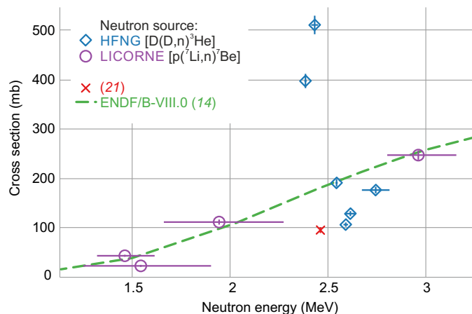
Fig. 3. Experimental cross section of the reaction ^{39}\text{K}(\text{n},\text{p})^{39}\text{Ar} as a function of neutron energy and their comparison with the most recent ENDF evaluation.
