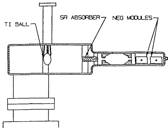
Figure 3. Vacuum chamber for the transition region [4] where the bend radius is only 45 m and the pressure must be held to less than 1 nTorr of CO and CO 2 .
