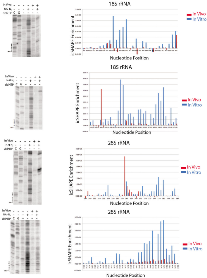
Extended Data Figure 4. icSHAPE is capable of reproducing RNA acylation profiles obtained by manual RNA modification experiments icSHAPE (right panels) profiles of ribosomal RNA and compared them to those obtained by manual SHAPE (left panels).
