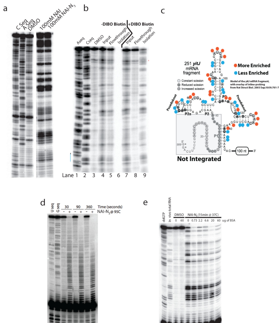
Extended Data Figure 3. NAI-N 3 is a novel RNA acylation reagent accurately reads out RNA structure
