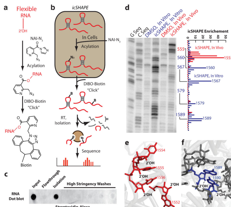
Figure 1. icSHAPE is a Novel and Robust Method for Measuring RNA Structure
