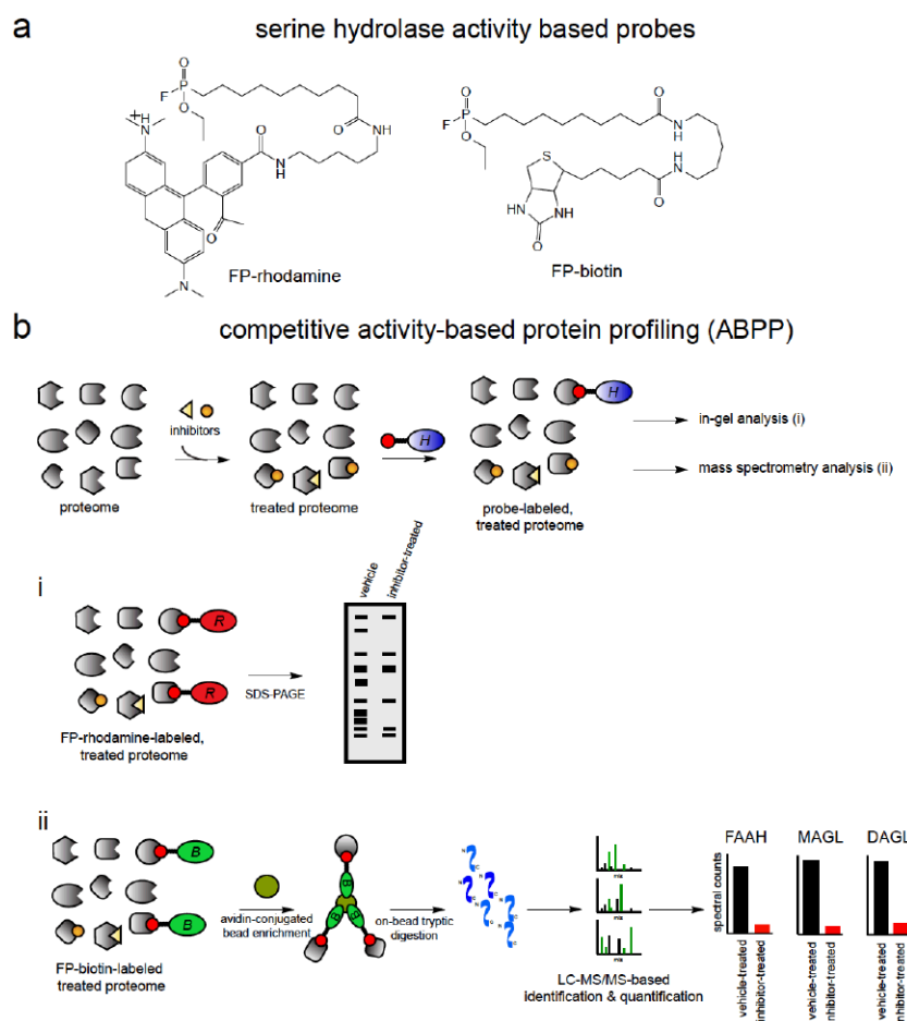
Figure 3. Activity-Based Protein Profiling (ABPP) for Developing MAGL and DAGL Inhibitors (a) Activity-based probes for serine hydrolases, fluorophosphonate (FP)-rhodamine and FP-biotin. (b) Competitive ABPP has been used to develop highly selective MAGL and DAGL inhibitors. ABPP uses active-site directed probes to assess the activities of large numbers of enzymes either by in-gel fluorescence (i) or by mass-spectrometry-based proteomics (ii). Because the probes bind to the active-sites, small-molecule inhibitor libraries can be competed against probe binding, facilitating an inhibitor-discovery platform. Selectivity can also be assessed across the entire enzyme class since probe-bound enzyme activities can be read-out in parallel.
