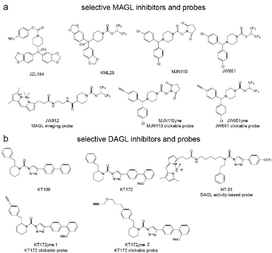
Figure 4. Selective MAGL and DAGL Inhibitors and Probes
