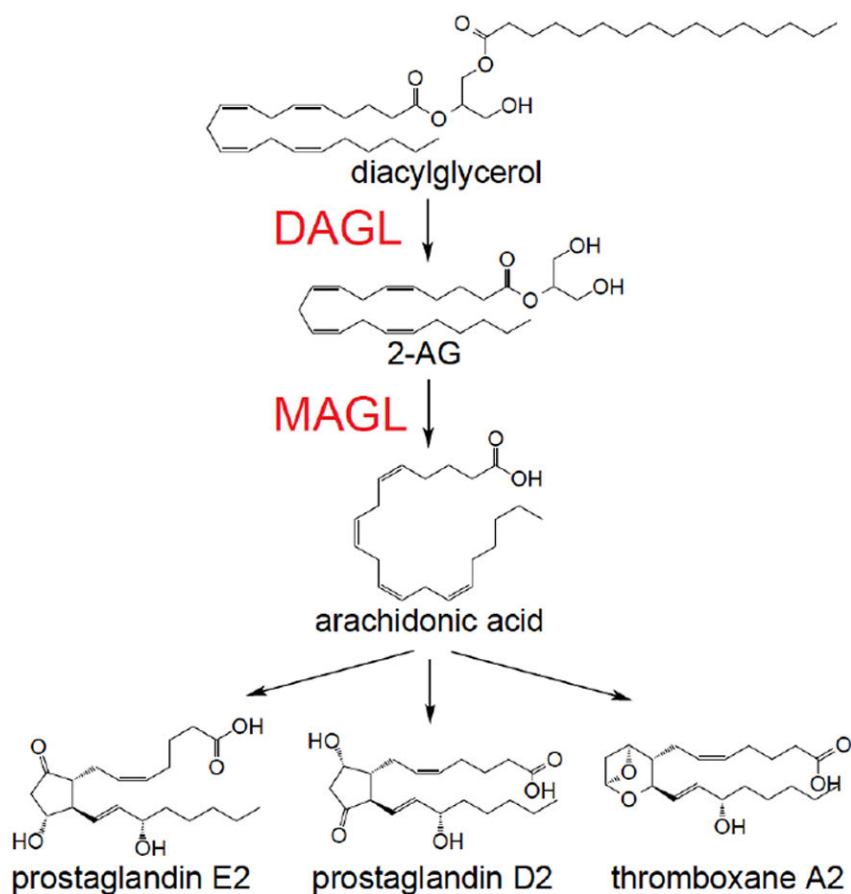
Figure 1. Pathways that Control 2-AG Degradation and Synthesis
