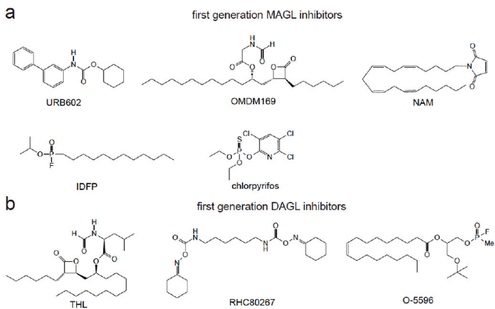
Figure 2. First-generation MAGL and DAGL Inhibitors
