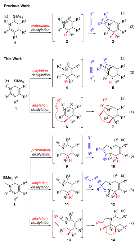
Figure 1. Endo- and exocyclic [3 + 2] cycloadditions via TMS dihydropyridines for the rapid synthesis of tropanes (eq 2-4), indolizidines (eq 5 and 7) and fused oxazolidines (eq 6).
