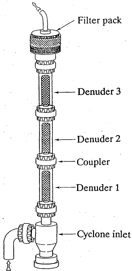
Figure 1. The integrated organic vapor-particle sampler in one field testing configuration. For some experiments the filter pack was placed after the first two denuders. The third denuder followed the filter pack.
