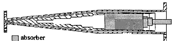
Fig. 4 TM_{om} waveguide-mode launcher
