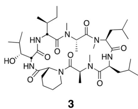
Figure 14. Compound 3.
