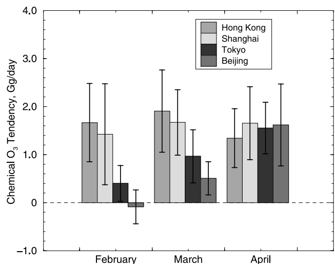
Figure 4. Net chemical O 3 tendency over four large metropolitan source regions in East Asia during spring 2001. See color version of this figure in the HTML.
