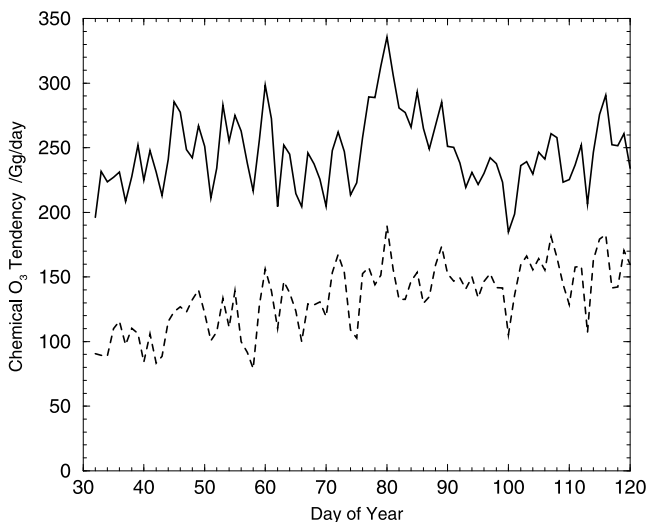
Figure 3. Daily net chemical O 3 tendency in the boundary layer (below 750 hPa) over the east Asian/western Pacific region (5°–45°N, 95°–150°E, solid line) and over China (22°–45°N, 100°–125°E, dashed) between February and April 2001, highlighting the daily variability and temporal trends over the period. See color version of this figure in the HTML.
