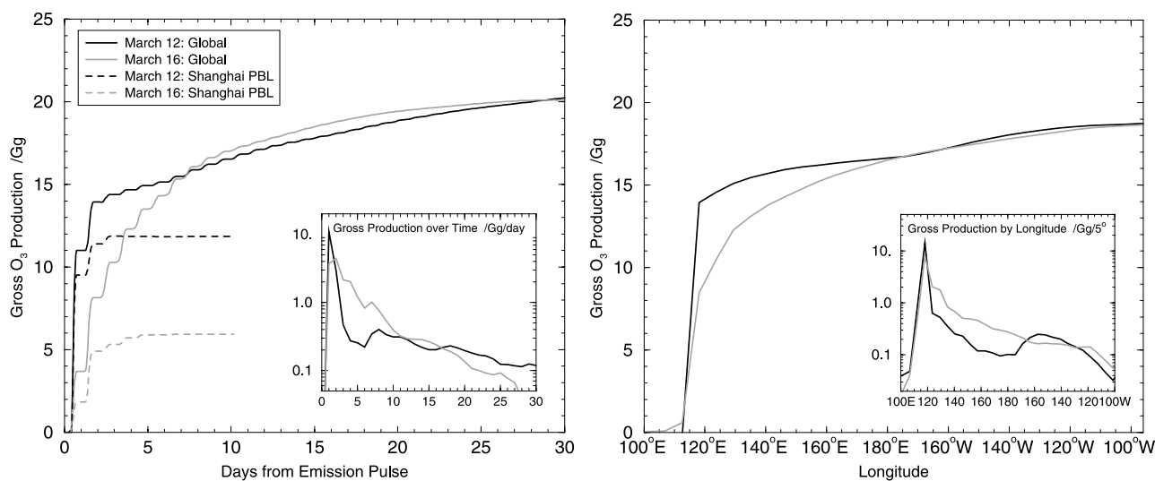
Figure 7. Cumulative additional O 3 formation (left) with time and (right) with longitude following 1 day's emissions of precursors from Shanghai on 12 March (black) and 16 March (grey), revealing the temporal and spatial evolution of gross production over the first month. Inserts show the absolute production on a log scale to highlight additional formation over the eastern Pacific after day 7 in the 12 March case.
