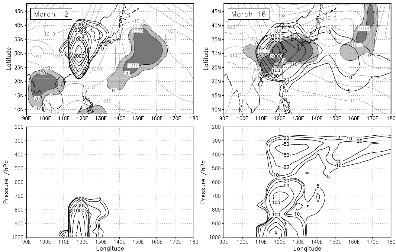
Figure 6. Column- and latitude-mean additional gross O 3 production (pptv) over the first 3 days following 1 day's emissions of precursors from Shanghai on (left) 12 March and (right) 16 March. Mean sea level pressure (grey contours) and cloud optical depth (shading) at the end of the first day are shown in the top panels. See color version of this figure in the HTML.
