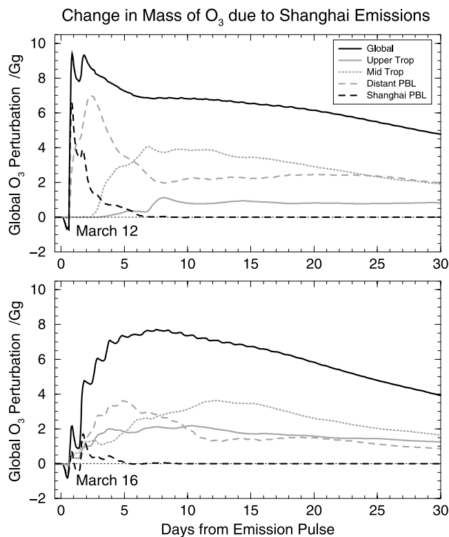
Figure 5. Additional mass of O_3 from 1 day's emissions of precursors from Shanghai on (top) 12 March and (bottom) 16 March. Note that the altitude regions are additive; together with the stratospheric impacts (which are small) they give the global perturbation. See color version of this figure in the HTML.
