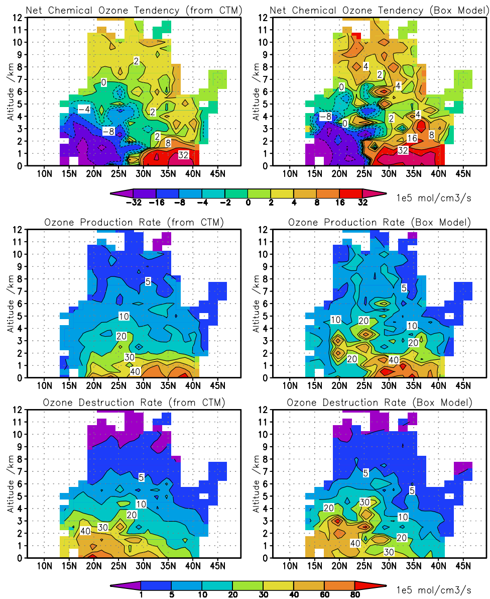
Figure 1. Net chemical O 3 tendency (10 5 molecules cm -3 s -1 , top) over the western Pacific (west of 145°E south of 30°N, west of 160°E north of 30°N) (left) from the CTM and (right) from steady state calculations constrained by aircraft measurements along flight tracks during the TRACE-P campaign. (bottom) Gross O 3 production and destruction rates. Note the different color scale used.
