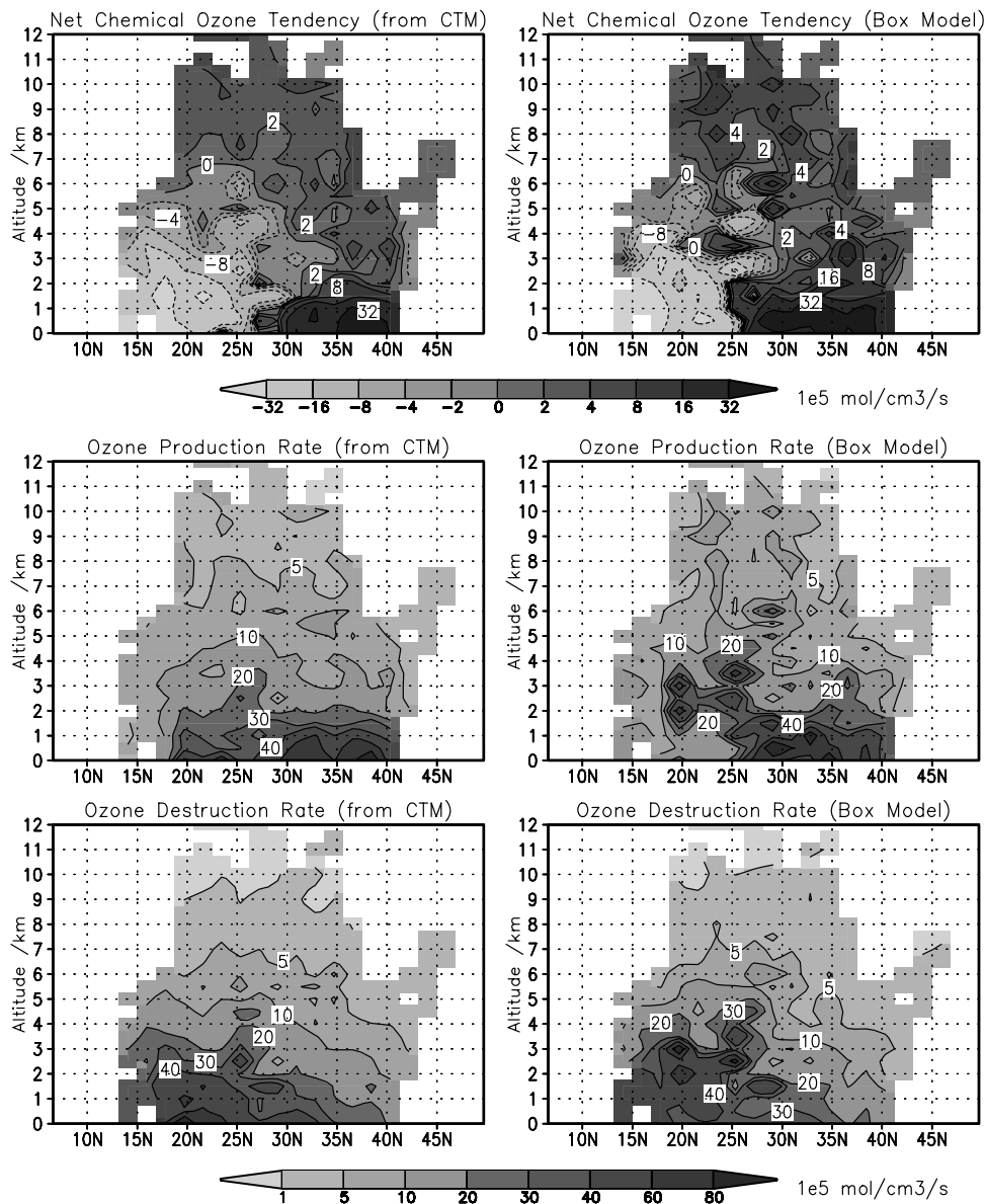
Figure 1. Net chemical O 3 tendency ( 10^5 molecules \text{cm}^{-3} \text{s}^{-1} , top) over the western Pacific (west of 145^\circ\text{E} south of 30^\circ\text{N} , west of 160^\circ\text{E} north of 30^\circ\text{N} ) (left) from the CTM and (right) from steady state calculations constrained by aircraft measurements along flight tracks during the TRACE-P campaign. (bottom) Gross O 3 production and destruction rates with a different color scale used. See color version of this figure at back of this issue.
