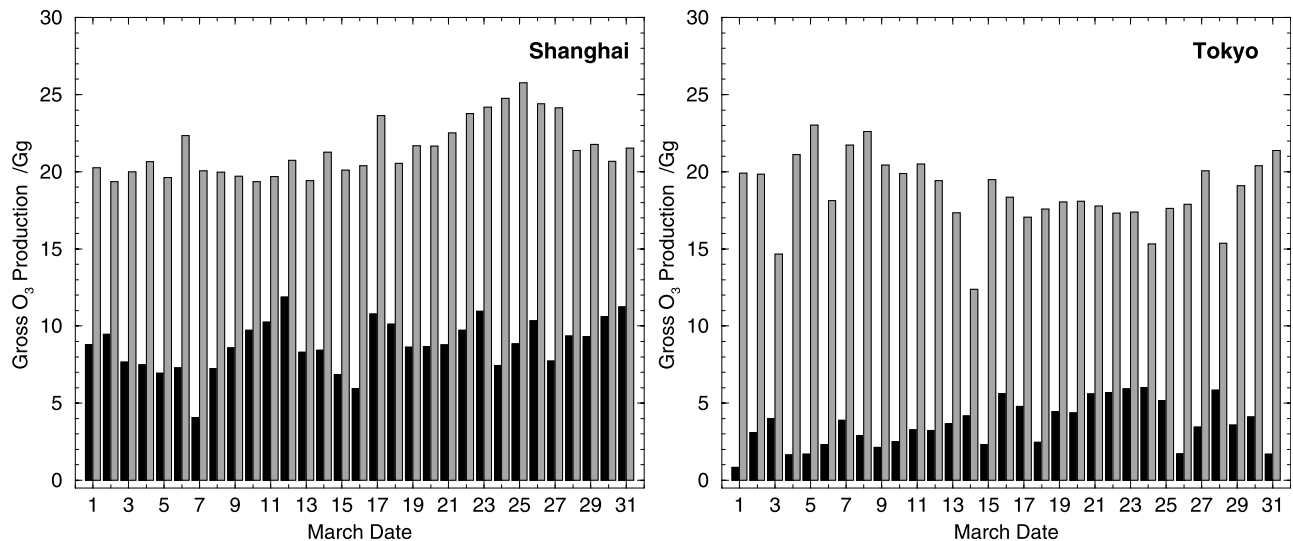
Figure 8. Additional gross O_3 production over one month over the source region (black) and over the globe (grey) following 1 day's emissions of precursors from Shanghai and from Tokyo for each day of March.
