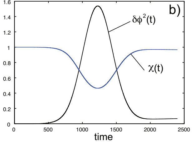
Figure 7: Ensemble level coherence correction. a) Time dependence of the adiabatic lower state population for Tully’s single crossing model. Exact wavepacket calculations (black) are compared with both the unmodified QTSH (blue) and QTSH + ensemble level decoherence corrected (cyan) results for initial momentum of \hbar k = 30 . Calculations are done in the adiabatic representation. b) Time dependence of the phase variance \delta\phi^2(t) and decoherence factor \chi(t) for the QTSH ensemble in a).
