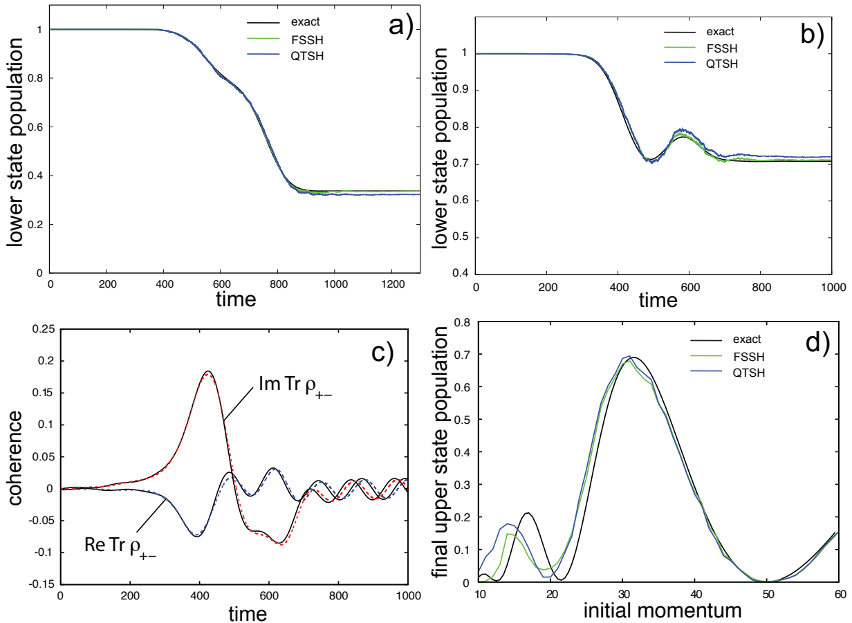
Figure 4: a) and b) Time dependence of the adiabatic lower state population for Tully's dual crossing model. The FSSH (green) and QTSH (blue) results are compared with exact wavepacket calculations (black). a) \hbar k = 30 . b) \hbar k = 40 . c) Coherence for \hbar k = 40 . Exact (black solid) and QTSH (dashed) results for the real (blue) and imaginary (red) parts of \text{Tr} \rho_{+-} are compared. See text for details. d) The final upper state population vs. initial momentum \hbar k is shown. Calculations are done in the adiabatic representation.
