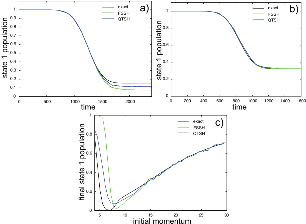
Figure 3: a) and b) Time dependence of the diabatic state 1 population for Tully’s single crossing model. The FSSH (green) and QTSH (blue) results are compared with exact wavepacket calculations (black). a) \hbar k = 10 . b) \hbar k = 15 . c) The final state 1 population vs. initial momentum \hbar k is shown. Calculations are done in the diabatic representation.
