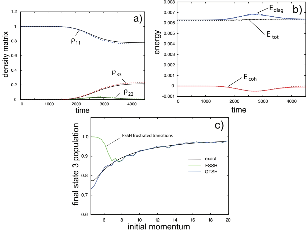
Figure 5: a) Time dependence of the the state 1, 2, and 3 populations for the superexchange model. QTSH (solid) is compared with exact wavepacket results (dashed). Initial momentum \hbar k = 5 . b) The energy budget for the \hbar k = 5 ensemble. c) Final state 3 population vs. initial momentum \hbar k . FSSH (green) and QTSH (blue) are compared with exact quantum results (black).
