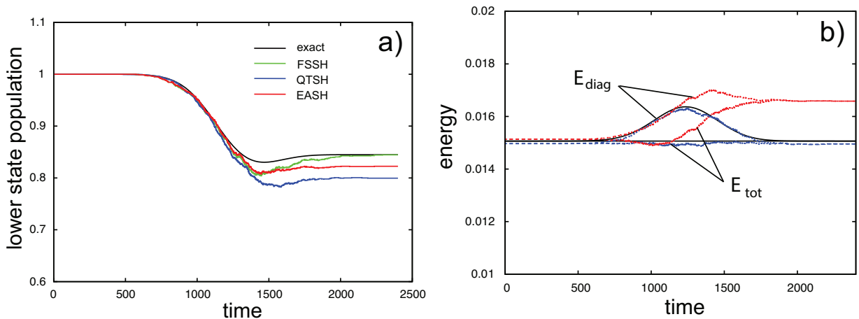
Figure 2: Comparison of FSSH and QTSH with an “energy aloof” variant, EASH. a) Time dependence of the adiabatic lower state population for Tully’s single crossing model with \hbar k = 10 . The FSSH (green), QTSH (blue) and EASH (red) results are compared with exact wavepacket calculations (black). b) The energy budget for the state is shown. Exact quantum results (black solid) are compared with the QTSH (blue) and EASH (red). The total E_{tot} and diagonal E_{diag} contributions are shown as a function of time. See text for discussion.
