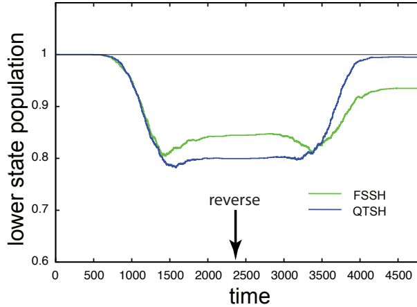
Figure 6: Time reversibility of surface hopping methods. The time dependence of the adiabatic lower state population for Tully’s single crossing model in the adiabatic representation are shown for the FSSH (green) and QTSH (blue) methods for initial momentum \hbar k = 10 . Simulation is run until t = 2400 (compare with Fig. 1) and then the signs of the momenta p_j and imaginary part of the coherence \beta_j are reversed for each member of the ensemble and the integration continued until t = 4800 .
