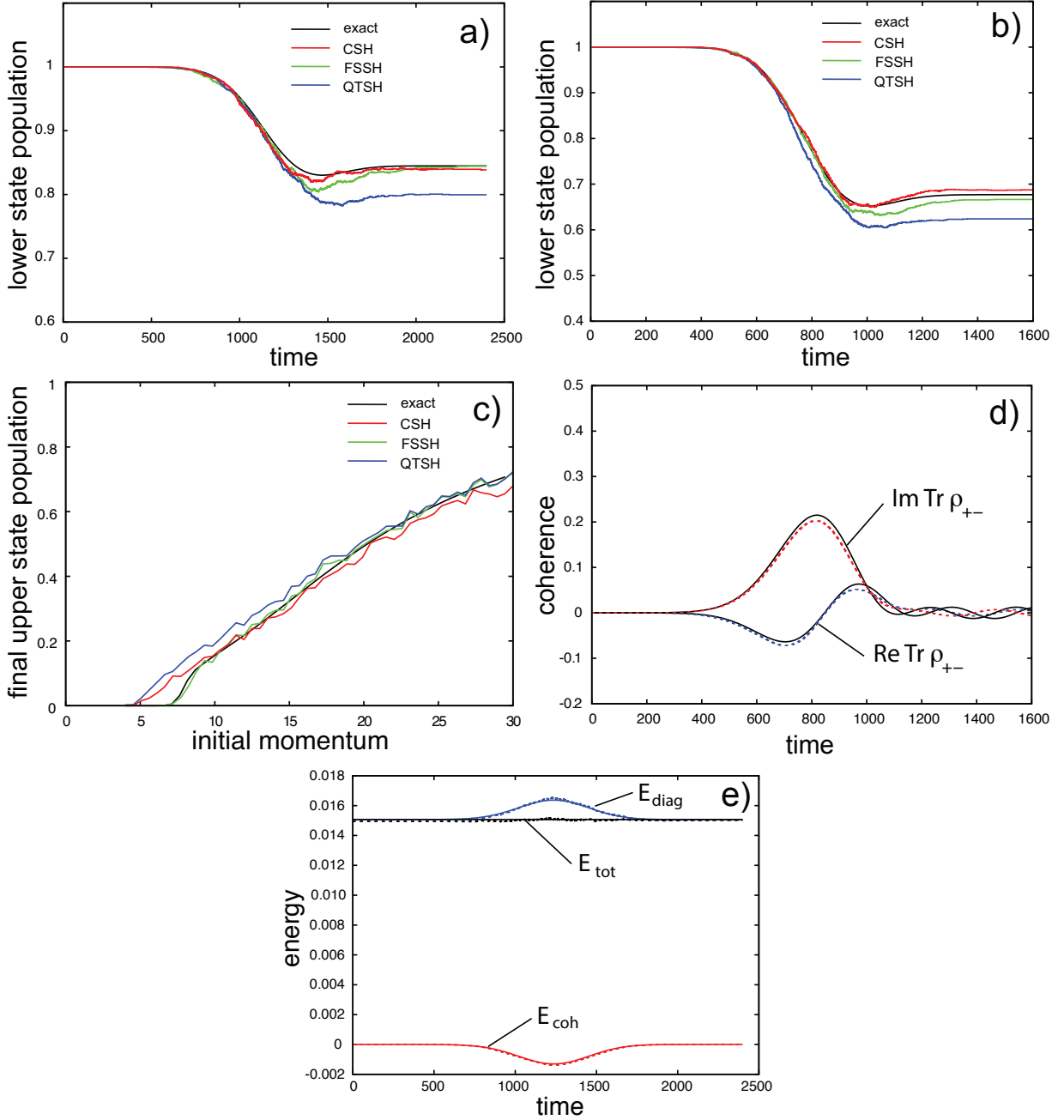
Figure 1: a) and b) Time dependence of the lower adiabatic state population for Tully's single crossing model. The FSSH (green), QTSH (blue) and CSH (red) results are compared with exact wavepacket calculations (black). a) \hbar k = 10 . b) \hbar k = 15 . c) The final upper state population is shown as a function of the initial momentum \hbar k . d) Coherence for \hbar k = 15 . Exact (black solid) and QTSH (dashed) results for the real (blue) and imaginary (red) parts of \text{Tr}\rho_{12} are compared. See text for details. e) The energy budget for the \hbar k = 10 state is shown. Exact quantum results (black solid) are compared with the QTSH ensemble (dashed colored). See text for discussion. Calculations are done in the adiabatic representation.
