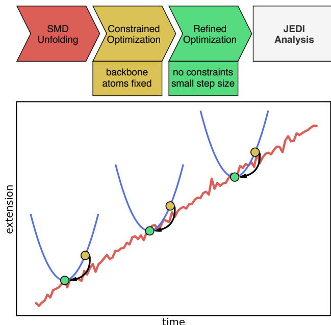
Figure 2: Schematic illustration of the applied workflow for JEDI analysis along the SMD unfolding trajectory. The upper part shows the individual steps toward JEDI analysis. The (non-quantitative) plot illustrates the SMD trajectory leading to a certain extension of the protein (red). Certain snapshots are extracted and quantum-chemically optimized keeping protein backbone atoms fixed (yellow dots). Then, the nearest local minimum, needed for JEDI analysis, is found through a constraint-free optimization of the previous geometry (green dot). In this manner, pairs of strained and relaxed structures along the unfolding trajectory are obtained, yielding a well-defined JEDI analysis per snapshot.
