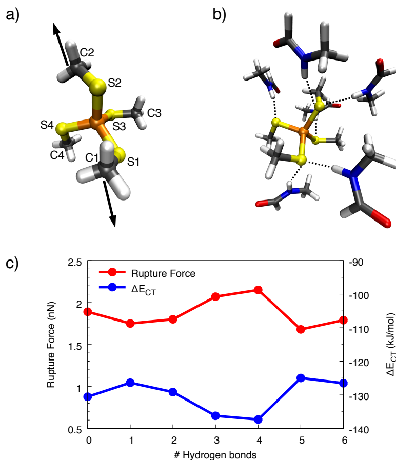
Figure 7: a) Simplified numbering scheme used in the quantum chemical model system. Stretching forces were applied to the carbon atoms C1 and C2. b) Quantum chemical model system with the complete set of formamide molecules forming hydrogen bonds (dotted lines) to the sulfur atoms of the \text{FeS}_4 unit. c) Rupture forces and charge-transfer energies \Delta E_{CT} calculated for the model system [\text{Fe(III)}(\text{SCH}_3)_4]^- with a varying number of hydrogen bonds formed between formamide molecules and the sulfur atoms. Lines were included to guide the eye.
