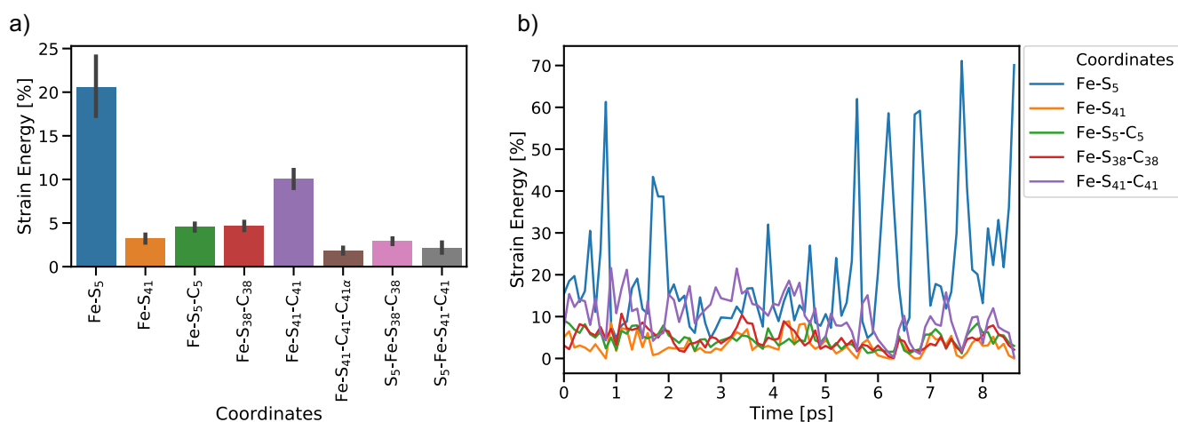
Figure 5: Summary of JEDI analyses including a) mean strain energy percentages for the most strained coordinates (bond lengths Fe–S 5 and Fe–S 41 , bond angles Fe–S 5 –C 5 , Fe–S 38 –C 38 and Fe–S 41 –C 41 , and torsions Fe–S 41 –C 41 –C 41α , S 5 –Fe–S 38 –C 38 and S 5 –Fe–S 41 –C 41 ) and b) time-resolved strain energy contributions (percentages of the total strain) of the most important bond lengths and bendings. Bars around the mean percentages indicate the 95% confidence interval.
