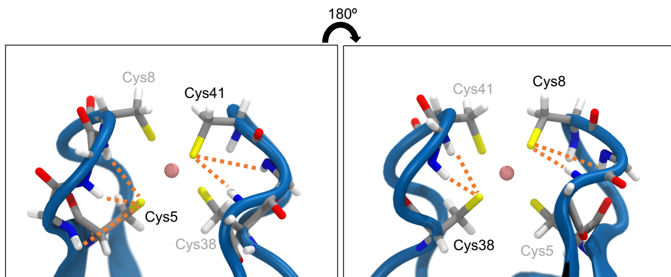
Figure 1: Close-up view of the central \text{FeS}_4 unit in rubredoxin (PDB 1BRF). Dotted lines represent possible hydrogen bonds between the sulfur atoms and the closest amino acid backbones (Cys5: Lys6, Ile7, Cys8; Cys8: Gly9, Tyr10; Cys38: Ile40, Cys41; Cys41: Gly42, Ala43) according to Ref. 18. The structure in the right panel is turned by 180^\circ w.r.t. the structure in the left panel.
