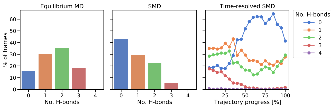
Figure 3: Analysis of protein hydrogen bonds to sulfur atoms of Cys5 and Cys41. The percentage of frames in which a certain number of hydrogen bonds occurs in equilibrium (left) and during the SMD unfolding procedure (middle). In the right panel, a time-resolved representation of hydrogen bond percentages is shown by averaging 20 equally sized trajectory windows. During the final parts of the trajectories, some of the Fe–S distances are already significantly elongated (cf. Figure S5).
