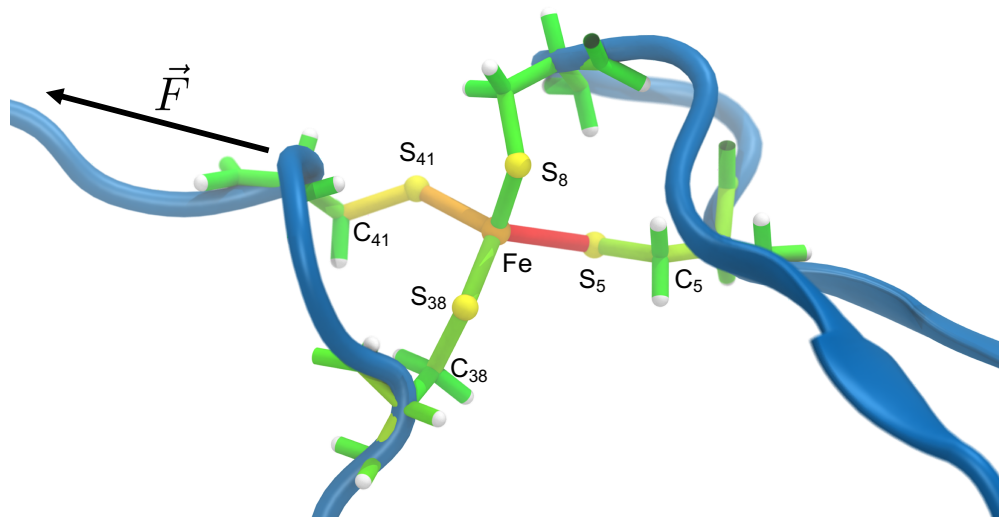
Figure 6: Representative snapshot of the unfolding trajectory before bond rupture. The strain energy contributions in the quantum region are mapped onto the bonds, where red and green indicate high and low strain, respectively, and transitions are fluent. The residues along the force coordinate bear most of the strain energy (Cys5 and Cys41), whereas Cys8 and Cys38 only play a minor role. The scissile bond Fe–S 5 contains most of the strain energy, followed by the angle on the opposite side (Fe–S 41 –C 41 ).
