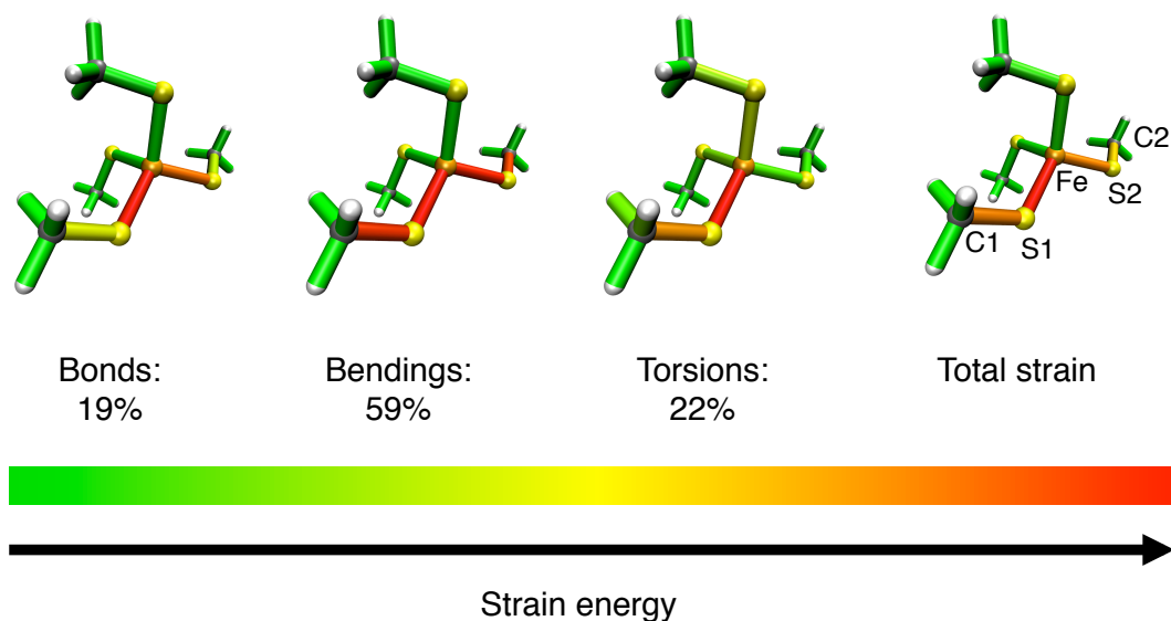
Figure 8: Color-coded distribution of harmonic strain energy among the bonds, bendings and torsions of [\text{Fe(III)(SCH}_3)_4]^- at a stretching force of 1 nN, as calculated with the JEDI analysis. The picture for the total strain includes the specification of the numbering scheme used to identify the strained bonds and bendings, which is a subset of the scheme specified in Figure 7B.
