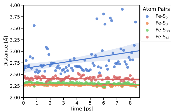
Figure 4: Fe–S distances of strained geometries before bond rupture. Subscripts indicate the amino acid residue number. Linear fits of the distances are displayed together with the confidence interval (translucent areas).
