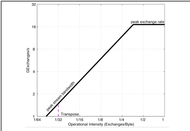
Figure 5. Roofline for transpose phase of 3-D FFT for the Cell
