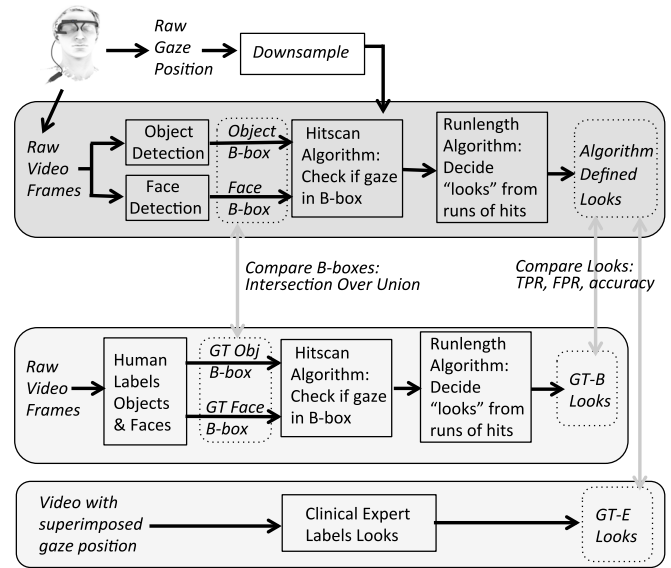
Fig. 1. Overview of the algorithm and GT formation. B-box stands for a bounding box, GT-B and GT-E are the two types of GT for looks, and TPR and FPR are true/false positive rates.
