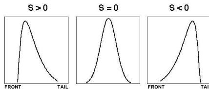
Fig. 1. Skewed pulse shapes characterized by the skewness parameter, S .
