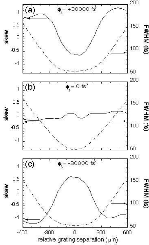
Fig. 2. Conventionally defined pulse width, FWHM (dashed curve) and skew, S , (solid curve) of ultrashort pulses in a CPA system plotted around the best compression in the function of the grating separation for three cases of third order bias phase components. (a): +30,000 \text{ fs}^3 , (b): 0 \text{ fs}^3 , (c): -30,000 \text{ fs}^3 .
