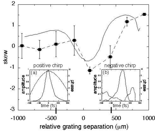
Fig. 3. Simulated (solid curve) and measured (squares) skew of pulses in a CPA system around the best compression plotted in the function of the grating separation. Inserts show retrieved amplitude and phase functions in the time domain at the marked relative grating separations. (a): -420 \mu\text{m} , positive chirp side, (b): +410 \mu\text{m} , negative chirp side
