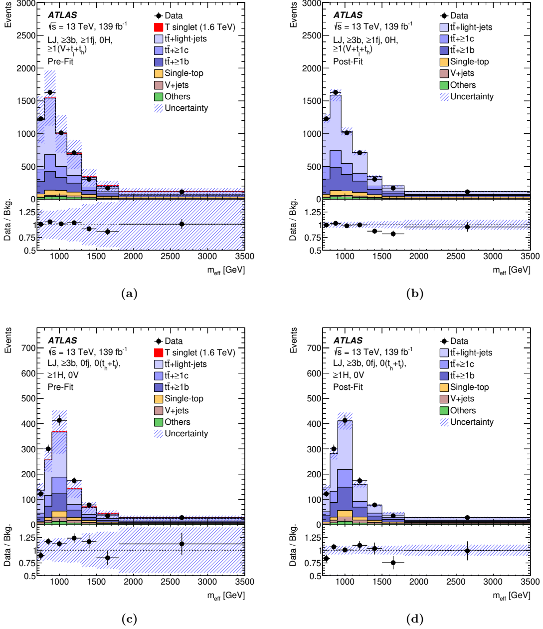
Figure 9. Comparison between the data and prediction for the m_{\text{eff}} distribution under the background-only hypothesis, in the (\text{LJ}, \geq 3b, \geq 1f_j, 0H, \geq 1(V+t_l+t_h)) validation region (a) pre-fit and (b) post-fit, and the (\text{LJ}, \geq 3b, 0f_j, 0(t_h+t_l), \geq 1H, 0V) validation region (c) pre-fit and (d) post-fit. The expected T singlet signal (solid red) for m_T = 1.6 TeV and \kappa = 0.5 is included in the pre-fit figures. The “others” background includes the t\bar{t} V/H, VH, tZ, t\bar{t}t\bar{t} , diboson, and multijet backgrounds. The bottom panels display the ratios of data to the total background prediction. The hashed area represents the total uncertainty in the background. The last bin in each distribution contains the overflow.
