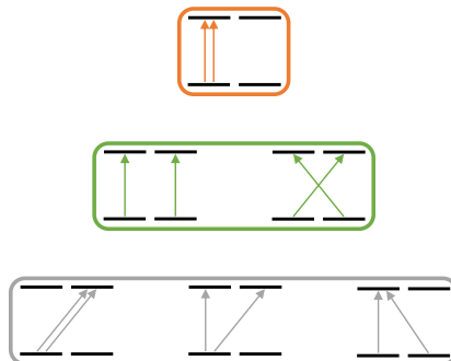
Figure 3: The three types of double excitations in MP2: on monomer (upper row), charge conserving (middle row), charge transferring (bottom row). Reprinted from [18], with the permission from AIP Publishing.
