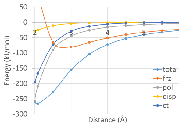
Figure 8: MP2/def2-TZVPP interaction energy components for C(NO_2)_3I \cdots F . [30] Reproduced by permission of the PCCP Owner Societies.
