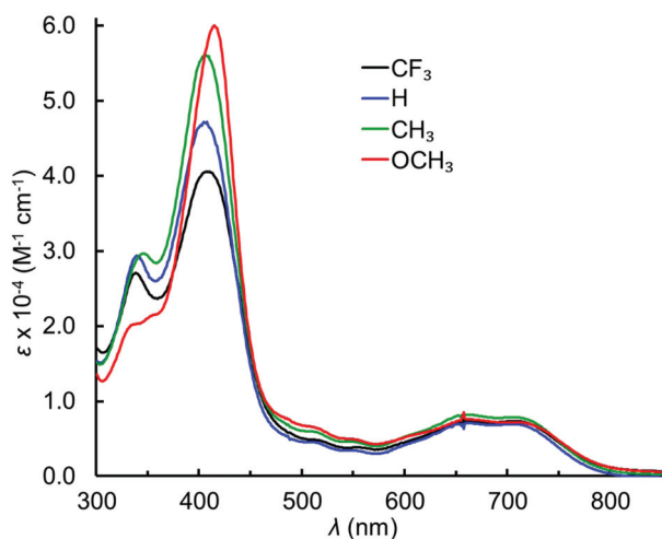
Fig. 4 UV-visible spectra of H 2 [5-pyr-TpXPIc], where X c {CF 3 , H, Me, OMe}.
