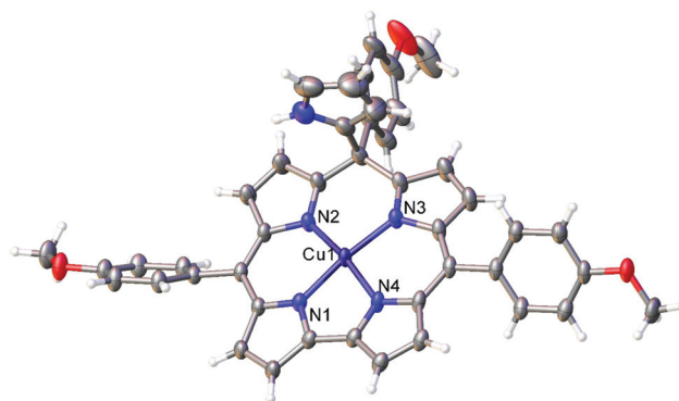
Fig. 3 Thermal ellipsoid plot for Cu[10-pyr-TpOMePiC]. Selected distances (Å): Cu1–N1 1.915(3), Cu1–N2 1.925(3), Cu1–N3 1.925(3), and Cu1–N4 1.921(3).
