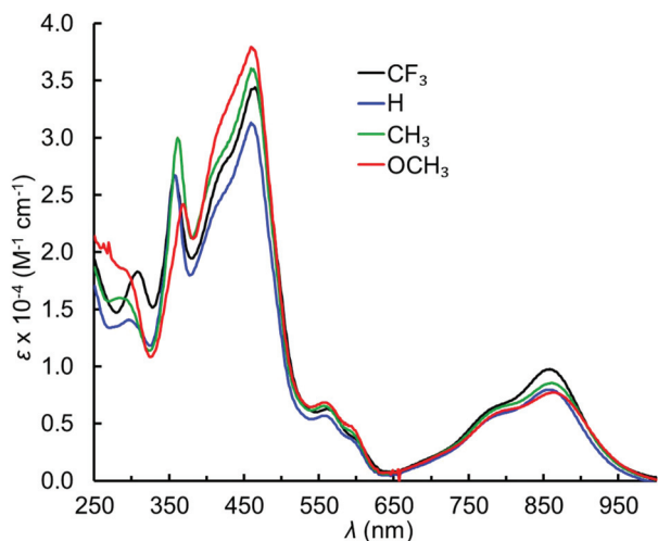
Fig. 6 UV-visible spectra of Cu[5-pyr-TpXPiC], where X c {CF 3 , H, Me, OMe}.
