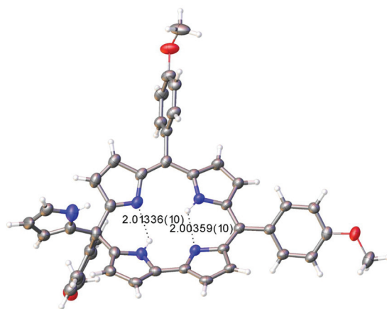
Fig. 2 Thermal ellipsoid plot for H 2 [5-pyr-TpOMePiC], including key hydrogen bond distances.
