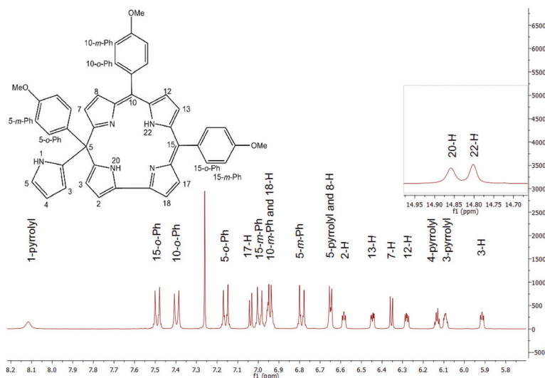
Fig. 1 The 1 H NMR spectrum of H 2 [5-pyr-TpOMePiC].
