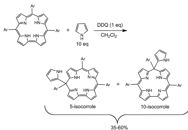
Scheme 1 Synthesis of pyrrole-appended meso -tris( para -X-phenyl) isocorroles, abbreviated hereafter as H 2 [5/10-pyr-TpXPiC], where X c (CF 3 , H, Me, OMe).
