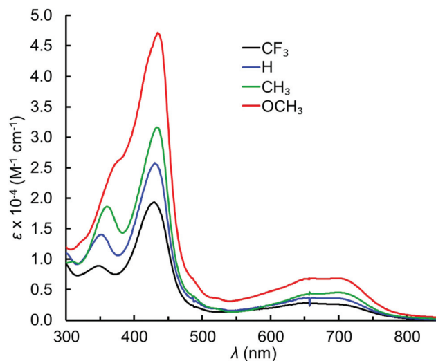
Fig. 5 UV-visible spectra of H 2 [10-pyr-TpXPIc], where X c {CF 3 , H, Me, OMe}.
