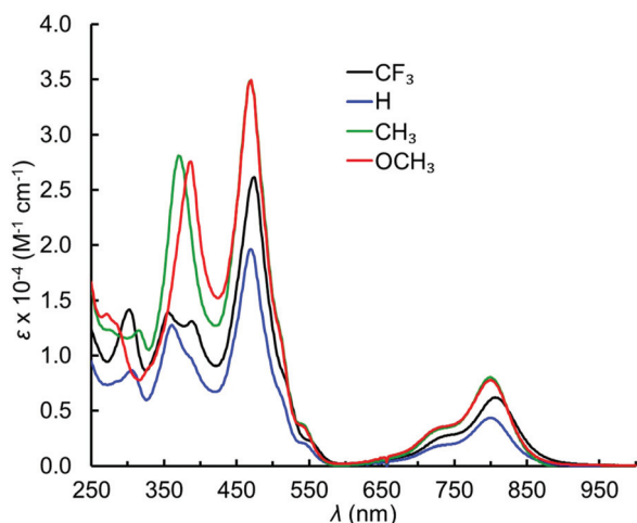
Fig. 7 UV-visible spectra of Cu[10-pyr-TpXPiC], where X c {CF 3 , H, Me, OMe}.
