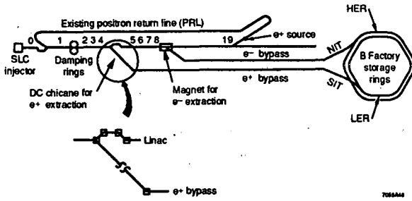
Figure 1. Schematic of the B Factory e^\pm injection system, based on use of the SLC linac with bypass lines. The numbers along the linac indicate the location (not to scale) of each sector. Each of the 30 sectors is 100 m long.
