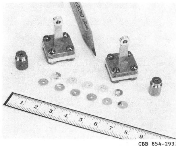
Figure 6 HGS Parts Prior to Assembly
