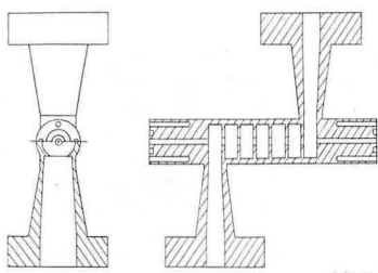
Figure 5 High Gradient Accelerator Test Structure (HGS)
