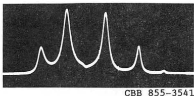
Figure 8 Transmitted Power vs Frequency for the HGS
