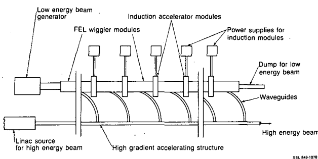
Figure 1 Two-Beam Accelerator
