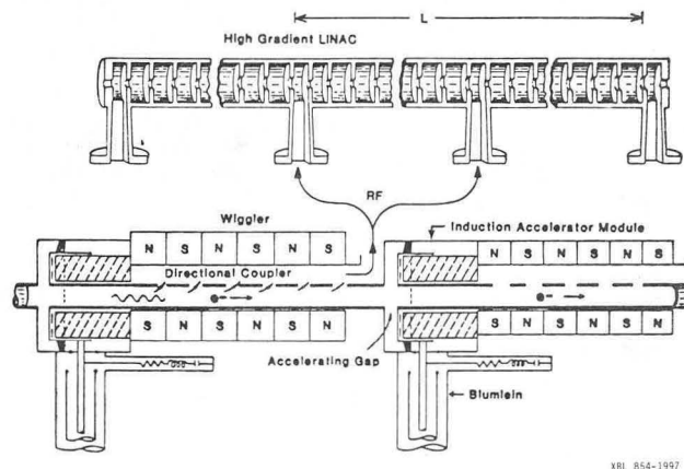
Figure 11 Early TBA Concept With Directional Coupling
