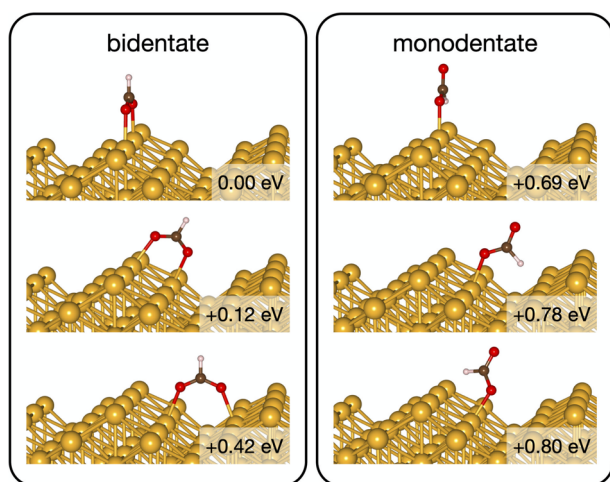
Fig. 7 The intermediate configurations of formate on Au(110)-1·2 categorized into two groups – bidentate and monodentate. The labelled relative energies are with respect to the most stable configuration. A more positive relative energy means a less stable structure.
