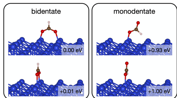
Fig. 8 The intermediate configurations of formate on Cu(110).
