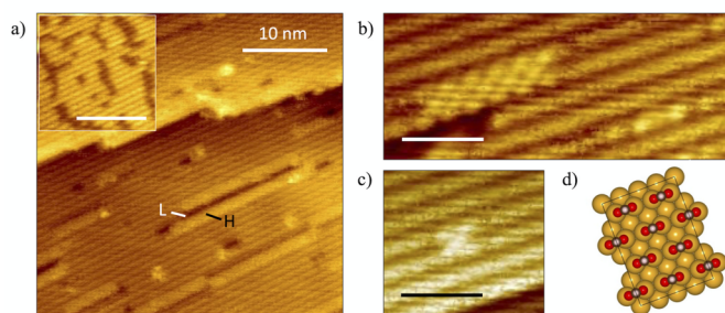
Fig. 6 Exposure of oxygen-covered Au(110) surface results in formation of formate clusters exhibiting a c(2 \times 2) structure and deconstruction of the underlying Au-(1×2) surface. (a) STM image showing formate condensation with inset showing the initial oxygen-covered surface at 0.08 ML. Surface was exposed to formic acid at 200 K. The surface lifetime of water and formic acid are less than a few seconds at this temperature, and only that of formate is significantly long for it to be imaged in these STM experiments; Scale bar in inset: 10 nm, image size: 35 \times 35 \text{ nm}^2 , sample bias: +1.5 V, tunneling current: 0.1 nA. The bright linear features (high-domains) are formate chains while dark linear features are lower domains of vacant neighboring Au rows descendent from the (1×2) reconstruction which were displaced. 65 (b) High-resolution STM image shows formate clusters along the close-packed rows and formate strings on unperturbed Au-(1×2). Image size: 4 \times 10 \text{ nm}^2 . (c) A single unit cell of c(2 \times 2) structure. Image size: 4 \times 4 \text{ nm}^2 . Scale bar in b) and c): 2 nm. d) Schematics illustrating the c(2 \times 2) formate structure on a deconstructed (1×1) Au surface.
