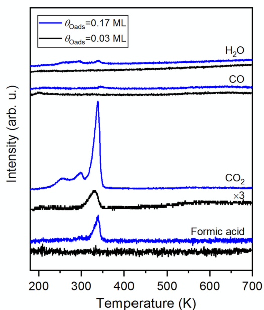
Fig. 1 The major product of temperature-programmed reaction of formic acid and oxygen-covered Au(110) is CO 2 ; small amounts of H 2 O and formic acid (HCOOH) are produced at higher coverages. 3 MLE of formic acid was dosed onto either 0.03 ML or 0.17 ML O/Au(110) at 200 K, above the desorption temperatures of unreacted molecular formic acid and H 2 O formed by the reaction between adsorbed oxygen species and acidic H of formic acid. Formic acid was also regenerated from the reaction between formate and hydrogen atoms released in formate decomposition. Heating rate was 1 K/s.
