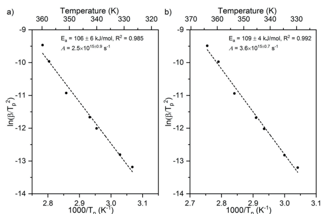
Fig. 5 Activation energy and pre-exponential factor of formate decomposition on Au(110) at formate coverages of a) 0.10 ML and b) 0.25 ML were determined by heating rate variation analysis. 6 The activation energy was 106 \pm 6 kJ/mol and pre-exponential factor was 2.5 \cdot 10^{15.0.9} \text{ s}^{-1} for 0.10 ML. The standard deviation for this coverage was higher than those for the other coverages. For 0.25 ML the activation energy was 109 \pm 4 kJ/mol and pre-exponential factor was 3.6 \cdot 10^{15.0.7} \text{ s}^{-1} . Formic acid was dosed onto oxygen-covered Au(110) at 250 K and heating rates of 0.2, 0.3, 0.7, 1, 2.2, 6, and 10 K/s were used.
