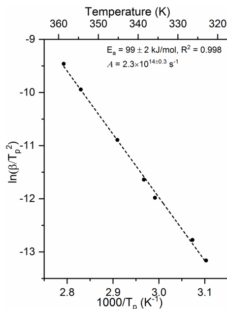
Fig. 4 Activation energy of 99 \pm 2 kJ/mol and pre-exponential factor of 2.3 \cdot 10^{14.0.3} \text{ s}^{-1} were obtained for 0.04 ML of formate decomposition on Au(110) by heating rate variation analysis. 6 Heating rates of 0.2, 0.3, 0.7, 1, 2.2, 6, and 10 K/s were used. Formic acid was dosed onto 0.02 ML O/Au(110) at 250 K. An E_a of 99 \pm 2 kJ/mol was obtained from the slope by least squares fitting and an A of 2.3 \cdot 10^{14.0.3} \text{ s}^{-1} was obtained by substituting E_a and pairs of \beta and T_p into Equation (3).
