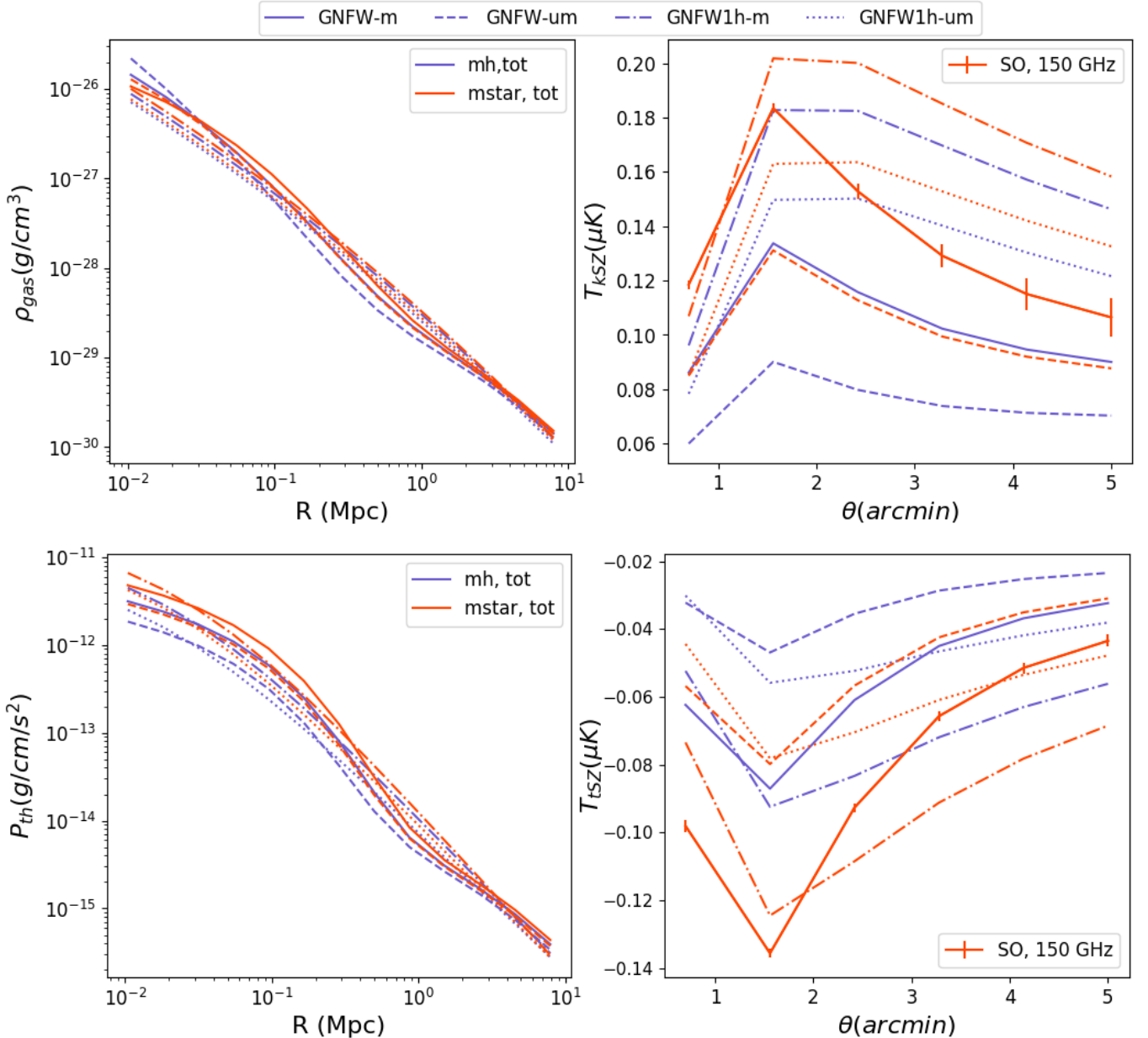
Figure 6. Projection process of M_{\text{OP-c-GT}} . Input 3D theoretical profiles (in this case, from TNG) and output the tSZ and kSZ observable temperature shifts as a function of radius in arcminutes. The different colors correspond to different mass selections, and different linestyles correspond to different fitting models and inclusion of distribution matching. The error bars correspond to the forecasted SO error bars at 150 GHz, discussed further in Section 3.3. These profiles show the effects of 1. selecting by different mass types, with the ‘ms’ samples having higher values and amplitudes than the ‘mh’ samples, 2. mass distribution matching, with more significant differences for pressure but still relevant for density, and 3. inclusion of a two-halo term, which results in lower amplitudes of the observed profiles as the 1h-only model overpredicts the values.
