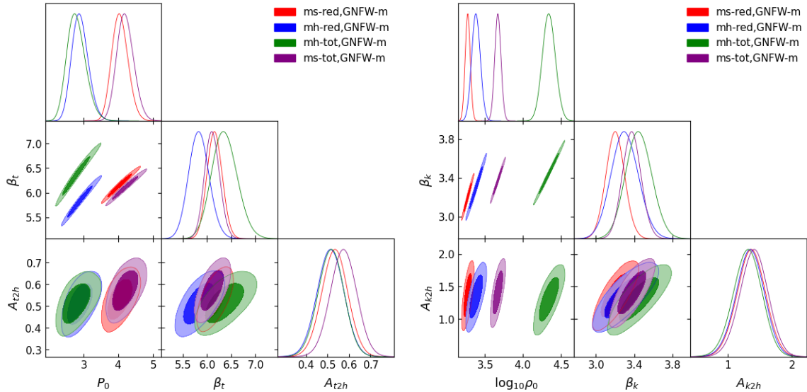
Figure 8. Comparison of parameter spaces for fits of the 2D projections of different samples, all for the GFW-m model. An additional parameter is fixed, x_{c,t} for pressure (left) and \alpha_k for density (right), as discussed in Section 4.3. This figure shows the differences among the fits of different samples (‘ms’ vs. ‘mh’, and ‘red’ vs. ‘tot’), highlighting the importance of these modeling choices.
