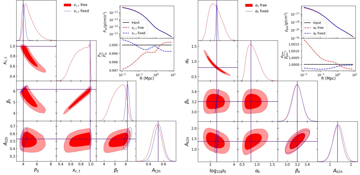
Figure 7. Contours for fits of projections for tSZ (left) and kSZ (right) for the GFW-m model of the ms-red samples. The contours for fits with all GFW parameters free are shown in red, and the contours for fits fixing an additional parameter are shown in blue. The vertical lines show the input parameter, the best 3D fit from the corresponding sample. The small panels show the 3D profiles computed using the corresponding values for each of the different contours, using a GFW model, and the same profiles normalized by the TNG profile to more clearly see the differences. This figure shows that the fits are not sensitive to information of the inner profiles, resulting in degeneracies, more significant for pressure. Fixing an additional parameter allows for better constraints on the remaining free parameters.
