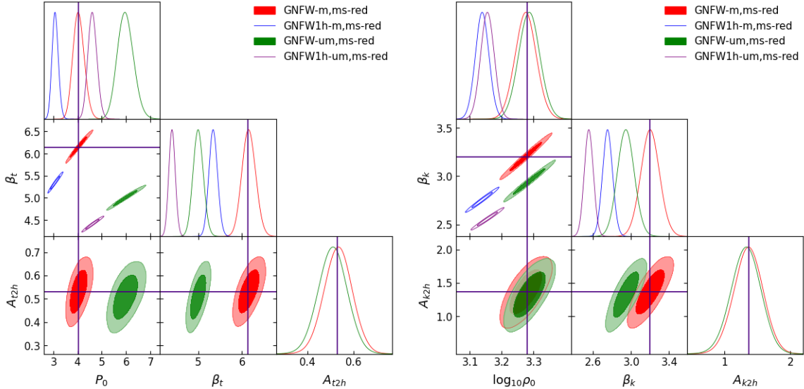
Figure 9. Comparison of parameter spaces for fits of the 2D projections ms-red sample with the GNFW-m model as the fiducial model. The solid lines indicate the values of the fits of the 3D profiles for the same sample (ms-red, GNFW-m). This figure shows that for density the most important modeling choice of the fitting model is the inclusion of a two-halo term, and for pressure both inclusion of distribution weighting and two-halo term are important.
