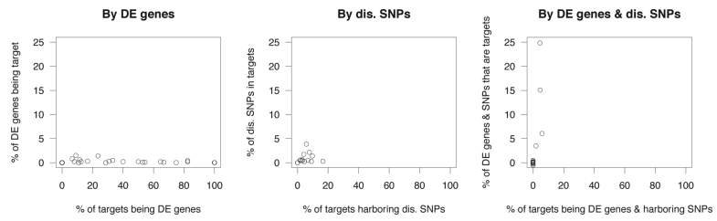
Figure 3. Performance of recovering known targets of each disease by DE genes, disease SNPs or both. Each point indicates the values of one disease.
