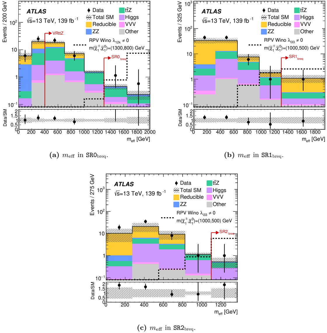
Figure 10. The m_{\text{eff}} distribution in (a) \text{SR0}_{\text{breq}} , (b) \text{SR1}_{\text{breq}} , and (c) \text{SR2}_{\text{breq}} for events passing the signal region requirements except the m_{\text{eff}} requirement. Distributions for data, the estimated SM backgrounds after the background-only fit, and an example SUSY scenario are shown. “Other” is the sum of the tWZ , t\bar{t}WW , t\bar{t}ZZ , t\bar{t}WZ , t\bar{t}WH , t\bar{t}HH , t\bar{t}tW , and t\bar{t}t\bar{t} backgrounds. The last bin captures the overflow events. The lower panel shows the ratio of the observed data to the expected SM background yield in each bin. Both the statistical and systematic uncertainties in the SM background are included in the shaded band. The red arrows indicate the m_{\text{eff}} selections in the signal and validation regions.
