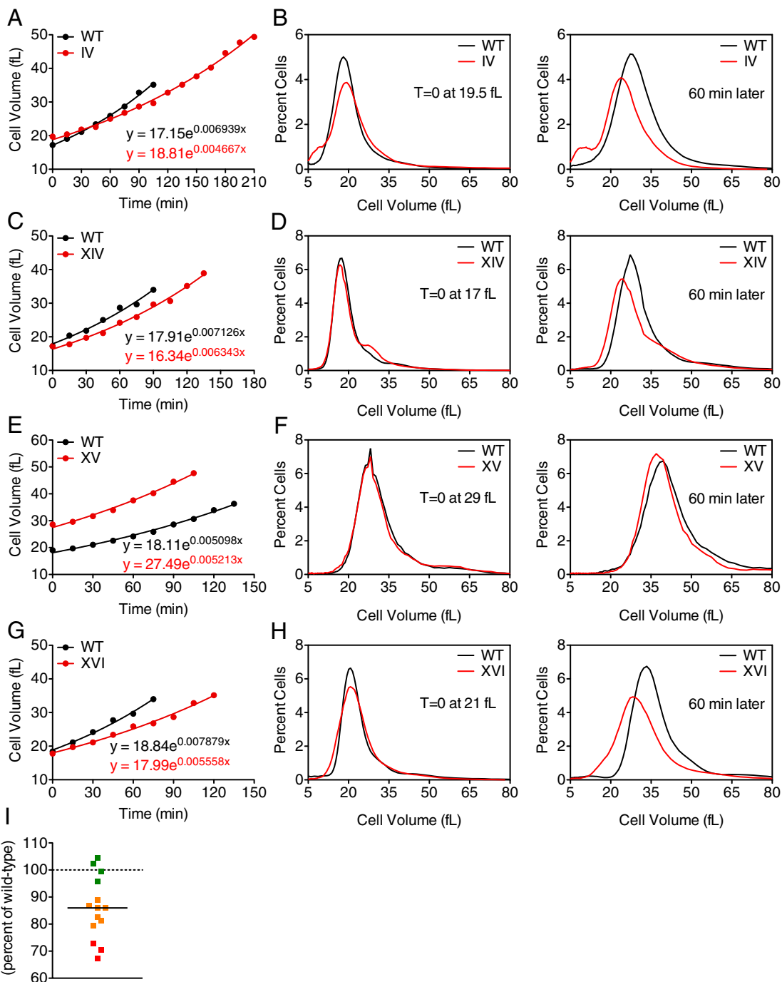
FIGURE 3: Cells carrying an extra chromosome show a decrease in growth rate during G1. (A–H) Wild-type (A–H; A11311, black), disome IV (A, B; A12687, red), disome XIV (C, D; A13979, red), disome XV (E, F; A12697, red), and disome XVI (G, H; A12700, red) cells were grown at 30°C in selective medium supplemented with 2% raffinose. Small, unbudded cells were isolated by centrifugal elutriation and released into the cell cycle at 30°C in YEPD. Time points were taken every 15 min to monitor cell volume. G1 time points (<20% budded cells in the population) were fitted to an exponential function to determine growth parameters. (B, D, F, H) Cell size distributions for elutriated wild-type (black) and disomic cells (red) of the same volume and after 1 h of growth in YEPD medium. (I) Distribution of growth constants for disomes II (A6865), IV (A12687), V (A14479), VIII (A13628), X (A21986), XI (A13771), XII (A12694), XIII (A21987), XIV (A13979), XV (A12697), XVI (A12700), XI + XV (A12691), XI + XVI (A12699), and VIII + XIV (A15615) are shown as the percentage of the wild-type (A11311) growth constant for each experiment. Disomes IV, XVI, and XI + XVI (red) show growth rates <75% of wild type; disomes V, VIII, XI, XII, XIII, XIV, and XI + XV (yellow) show growth rates 75–90% of wild type; and disomes II, X, XV, and VIII + XIV (green) show growth rates 90–110% of wild-type.
