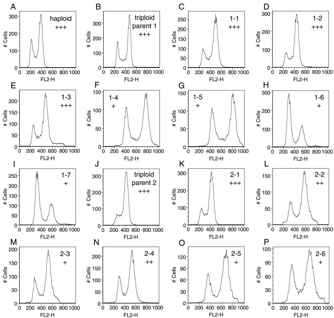
FIGURE 11: Progeny of triploid meioses exhibit a G1 delay. MATa/a/α (B; triploid parent 1, A6424) and MATa/a/α (J; triploid parent 2, A6425) cells were induced to sporulate, and tetrads were dissected. Individual colonies were picked after 1 wk and grown to exponential phase in YEPD medium to determine DNA content (C–I; A6424 progeny; K–P; A6425 progeny). FL2-H detection thresholds were adjusted for each strain so that the cell population was within the linear detection range of the instrument. Plus signs indicate proliferation rates on solid medium, with +++ representing proliferation rates close or equal to wild-type controls and fewer plus signs indicating poorer proliferation rates. A haploid strain (A2587) is shown in A.
