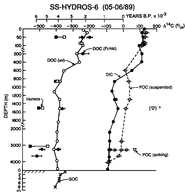
Fig. 2. \Delta^{14}\text{C} measurements of \text{DOC}_{uv} , \text{DOC}_{FI-hlc} , humic materials, suspended POC, sinking POC, DIC and sedimentary organic carbon (SOC) from the Hydros-6 cruise in the SS. Solid squares are XAD-2 isolates and open squares are XAD-4 isolates. Bars on \text{DOC}_{FI-hlc} represent errors of the \Delta^{14}\text{C} measurements; the error of all other measurements are included in the size of the symbols.
