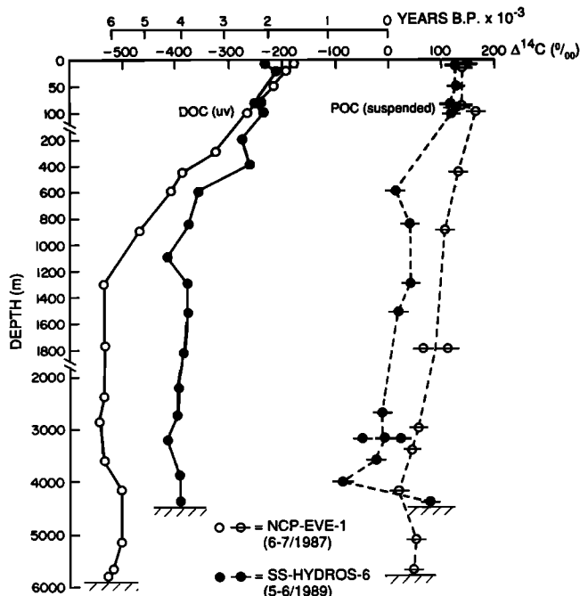
Fig. 6. A comparison of the \Delta^{14}\text{C} measurements for \text{DOC}_{uv} and suspended POC from the North Atlantic (Hydros-6) and the NCP (Eve-1) sites.
